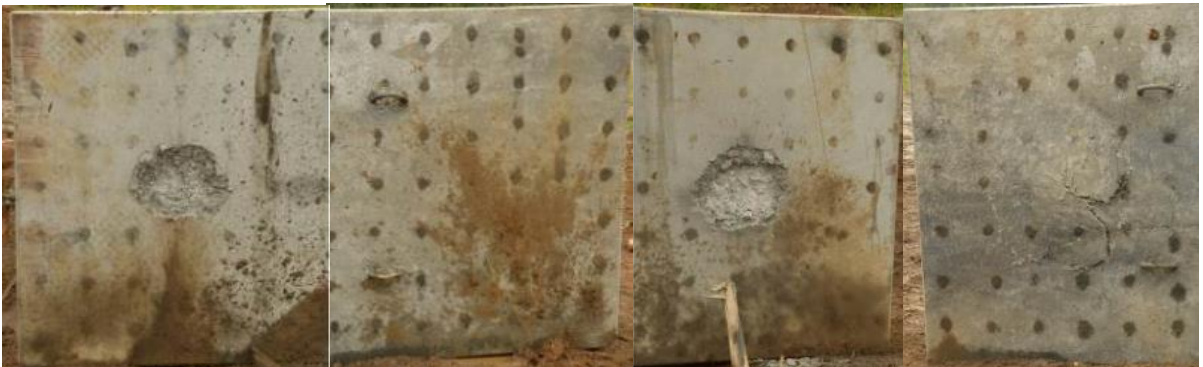
Figure 3. Specimen No. 13 after contact blast loading, 0.5 kg charge left left contact side, left right soffit, 1.4 kg charge right left contact side, right right soffit
