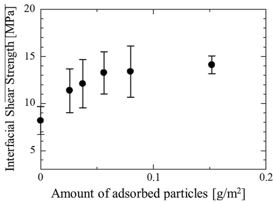
Fig. 5. Effect of particle amounts adsorbed on the modified carbon fibers on the interfacial shear strength.
