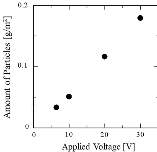
Fig. 4. Effect of applied voltage on the amount of PMMA particles adsorbed on the carbon fibers.
