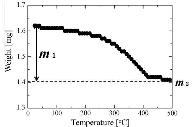
Fig. 2. TG curve of the modified carbon fibers with PMMA particles.
