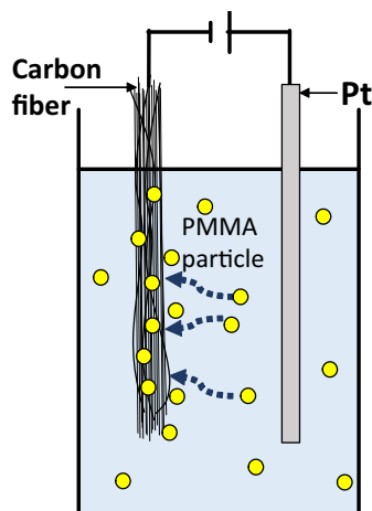
Fig. 1. Adsorption on carbon fiber system using polymer colloid and electrophoresis. (For interpretation of the references to color in this figure legend, the reader is referred to the web version of this article.)
