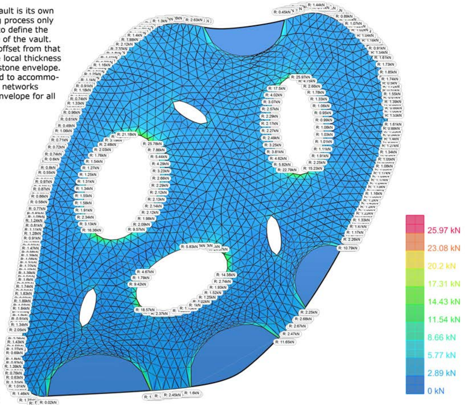
vault plan - load calculation
