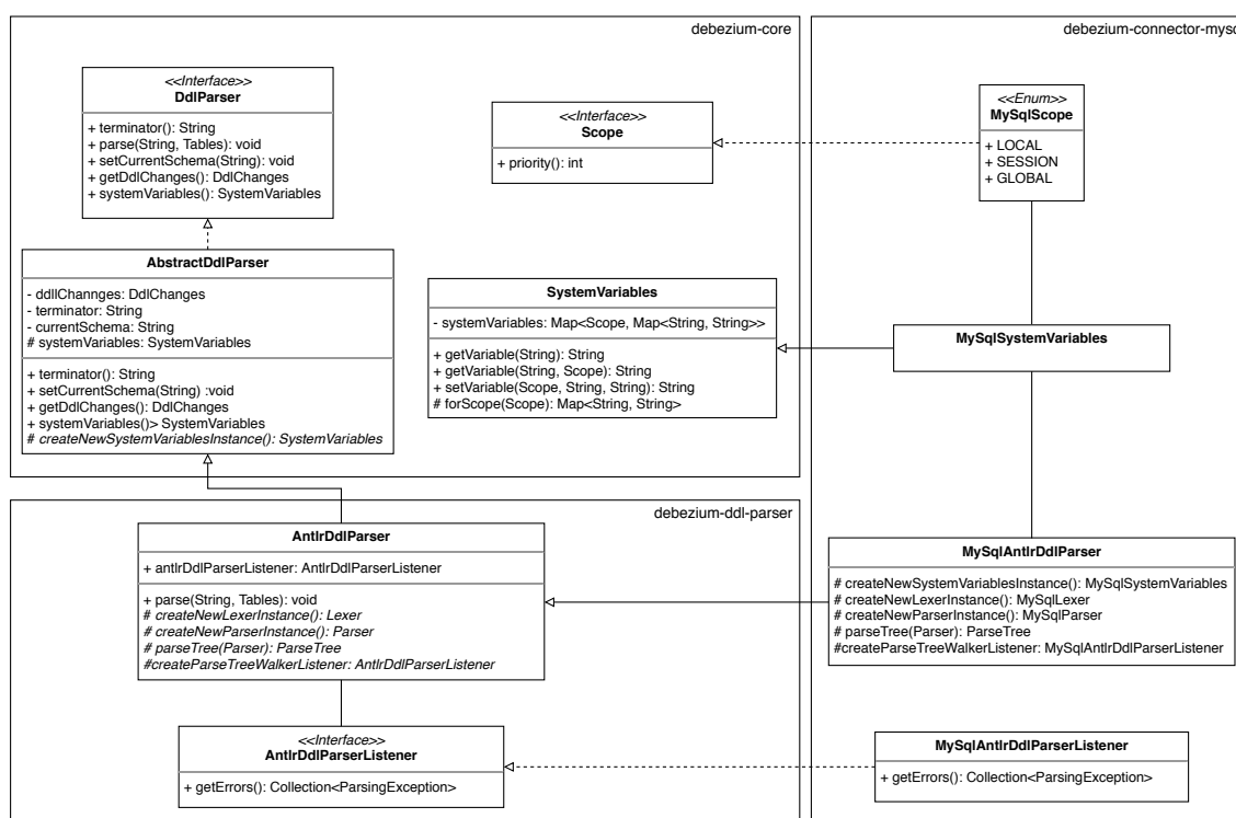
Obr. 6.3: Diagram tried MySQL ANLTR DDL parseru
