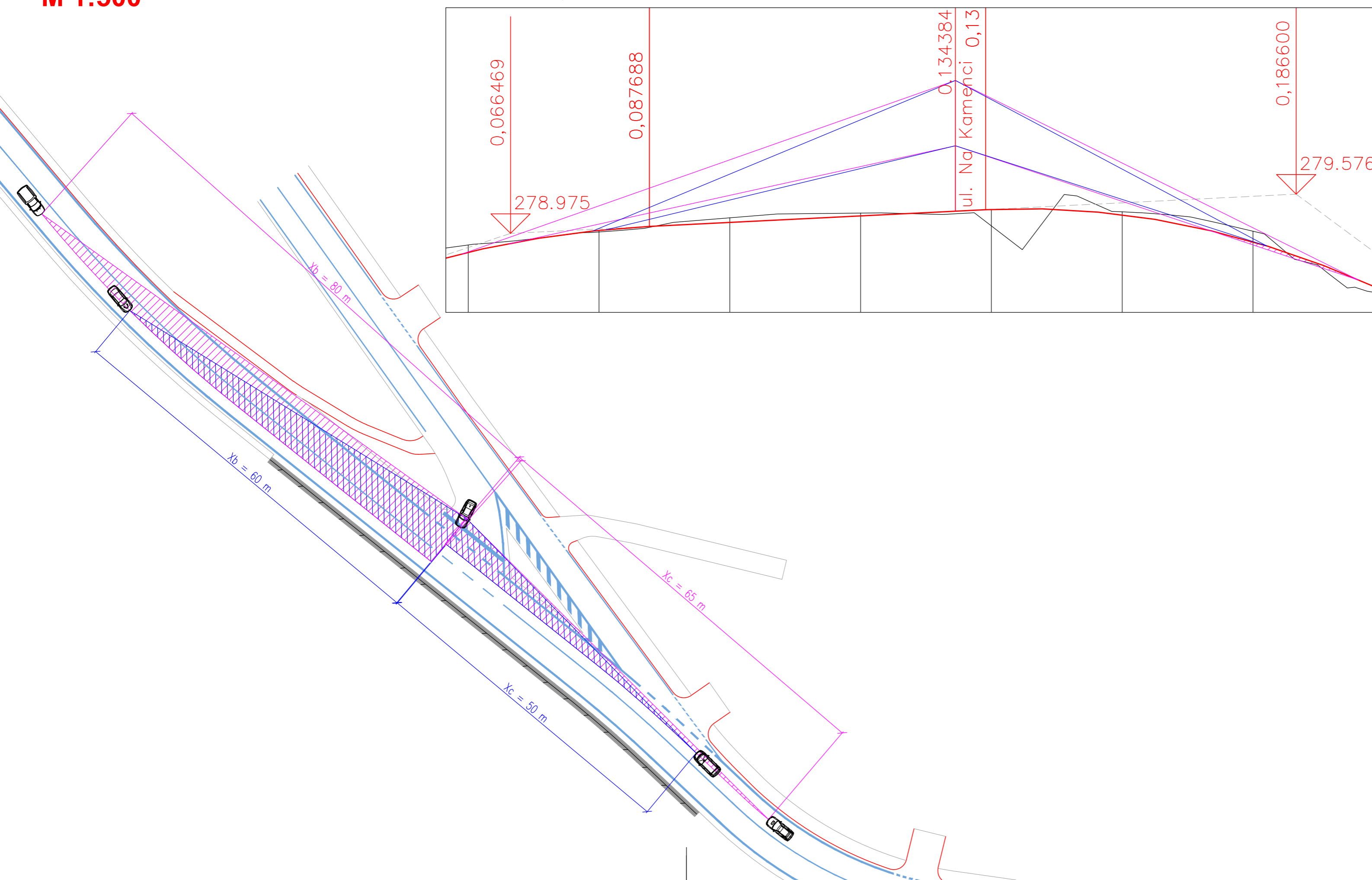
DETAIL A, M 1:500/50
