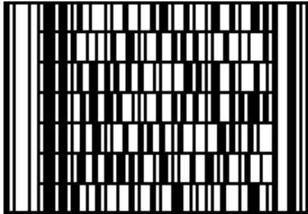
Codablock-F
