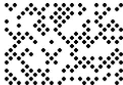
DotCode
