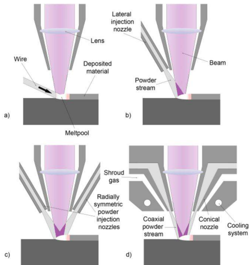
Figure 10.2: Different feeding mechanisms [10]
