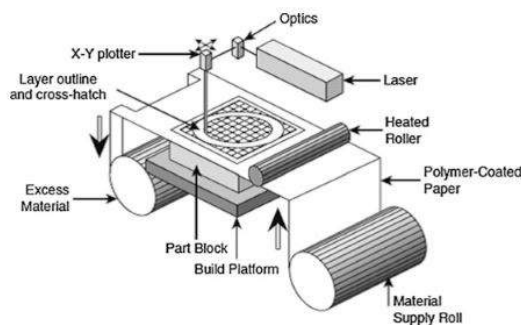
Figure 9.1: Bonding, followed by shaping, [1, p. 220]
