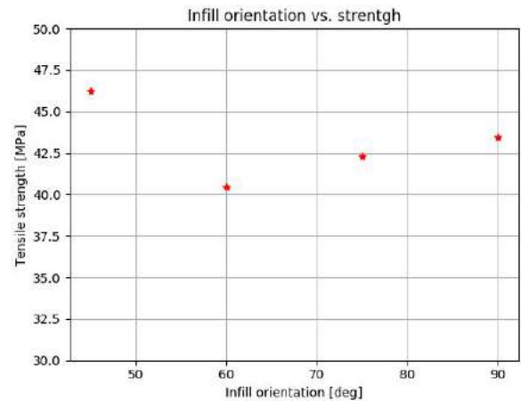
Figure 11.6: Effect of changing infill orientation on tensile strength
