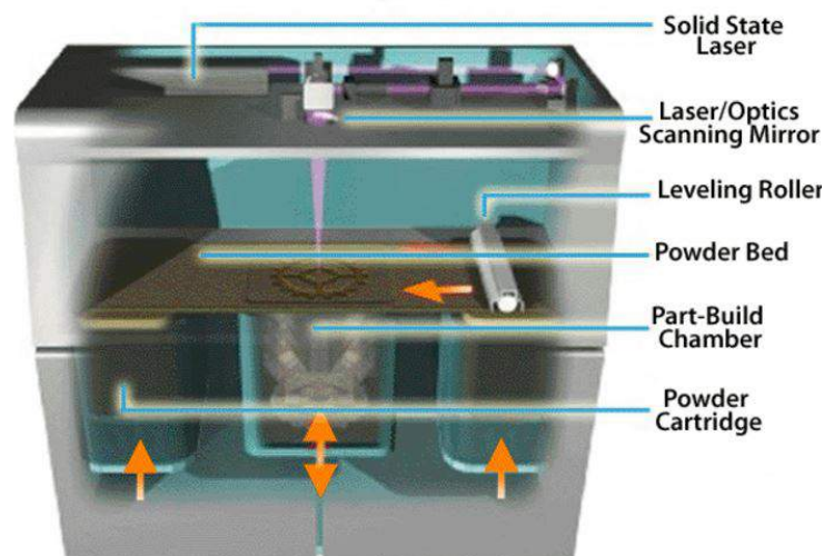
Figure 5.1: Real PBF machine, showing all necessary utilized equipment, [32]
