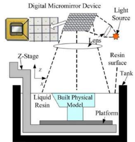
Figure 4.2: Utilizing Digital micromirror with SLA, [11]
