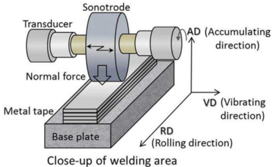
Figure 9.3: Schematic of ultrasonic metal welding SL machine, [33]
