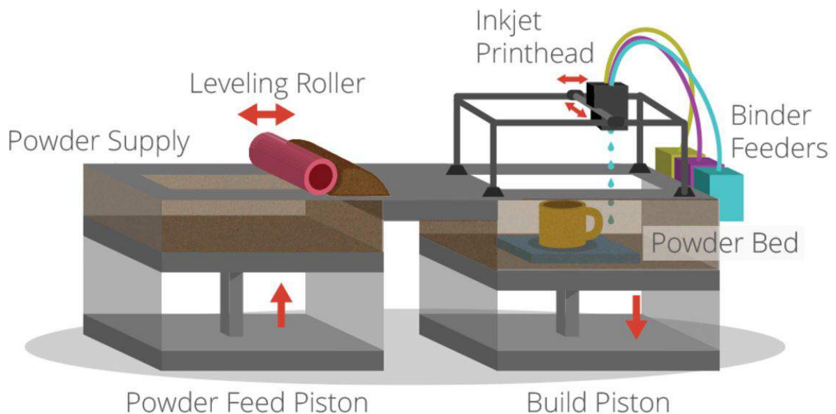
Figure 8.1: Schematics of a basic BJ machine, [23]
