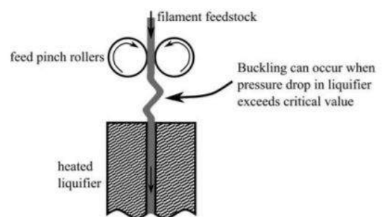
Figure 6.2: Illustration of filament buckling [16]
