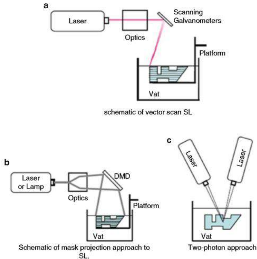
Figure 4.1: Illustration of SLA technologies, [1, p. 65]
