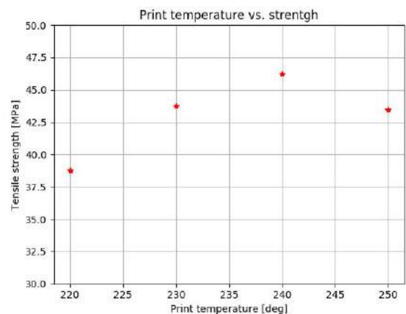
Figure 11.8: Effect of print temperature on tensile strength
