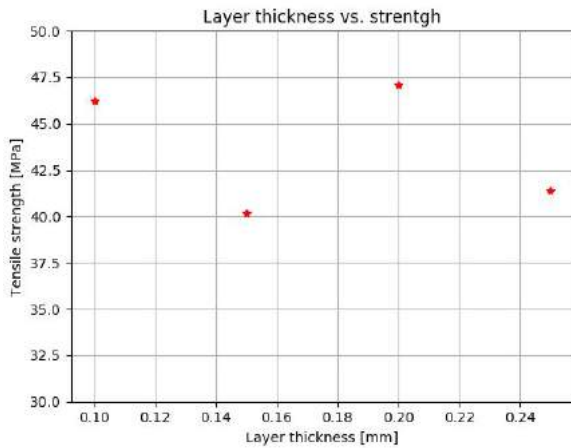
Figure 11.5: Effect of changing layer thickness on tensile strength
