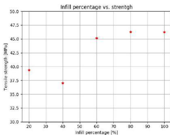
Figure 11.7: Effect of infill percentage on tensile strength
