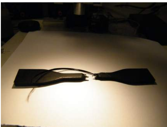
Figure 11.13: Elongation of single thread, separated from part during stressing
