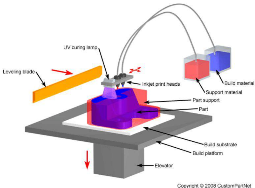
Figure 7.1: Common MJ machine setup [20]
