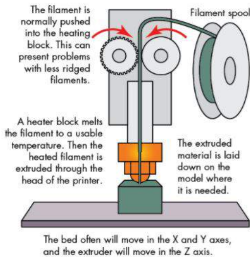
Figure 6.1: Common machine setup with pinch roller, [8]
