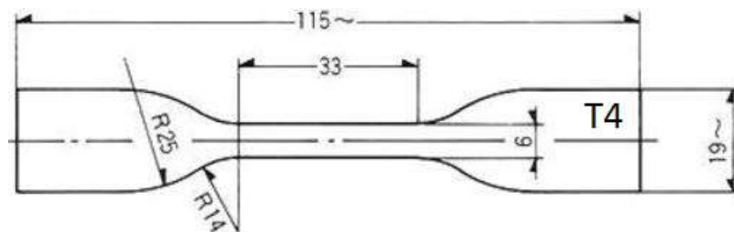
Figure 11.1: ASTM D638 - dimensions of test specimen type 4
