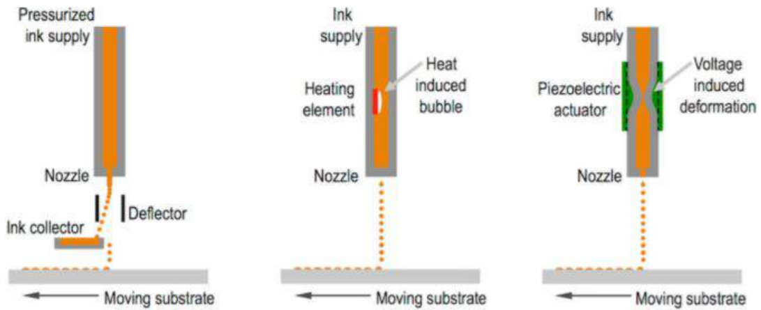
Figure 7.2: Continuous and thermal / piezoelectric drop-on-demand deposition [26]
