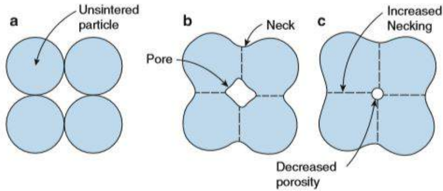
Figure 5.3: Illustration of particle fusion and necking process, [1, p. 113]
