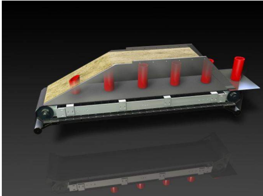
Figure 8.2: Voxeljet continuous printing on an inclined plane [25]
