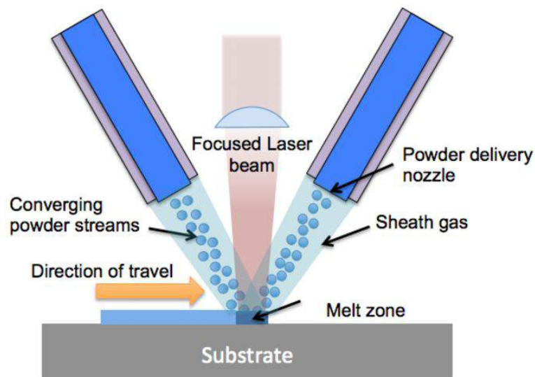
Figure 10.1: Common DED machine setup, using laser and powder feeding, [31]
