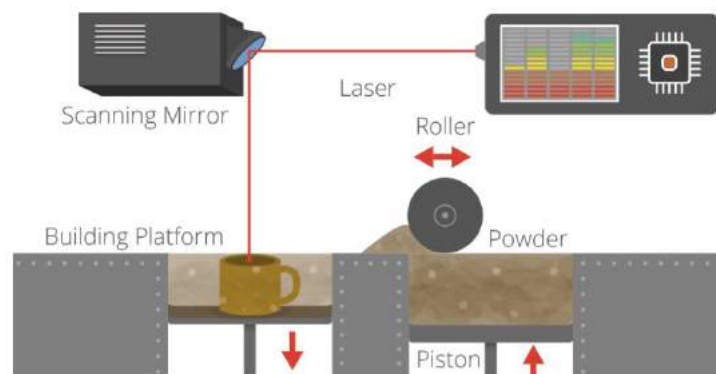
Figure 5.2: Illustration of roller spreading mechanism, [14].
