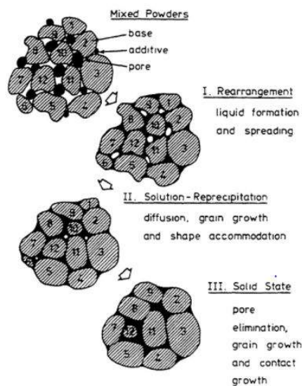
Figure 5.4: Liquid phase sintering of separate particles mixture, [17, p. 6]
