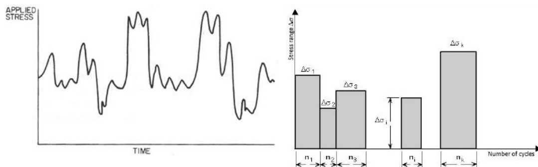
Figure 2.11: An example of variable amplitude loading and stress histogram resulting from the application of cyclic counting method (Al-Emrani et al., 2014).
