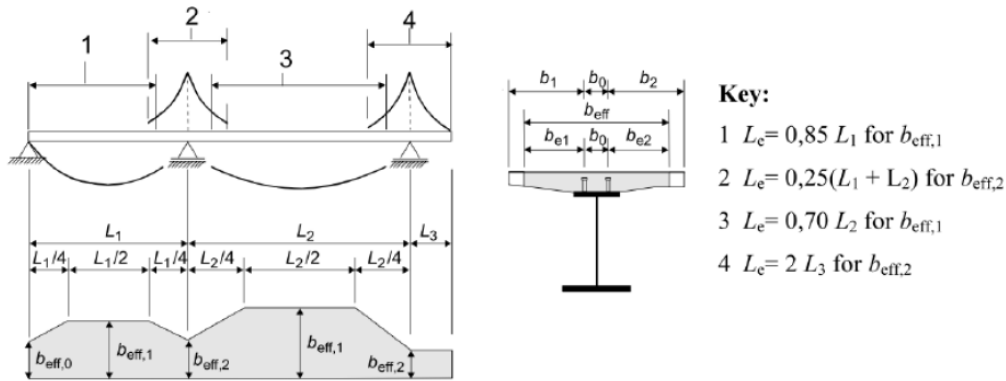
Figure 3.3: Equivalent spans, for effective width of concrete flange (EN 1994-2).
