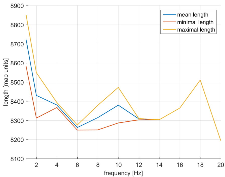
Figure 12.5.: Re-sampling and optimization results graph. This is visualization of data from table 12.1.
