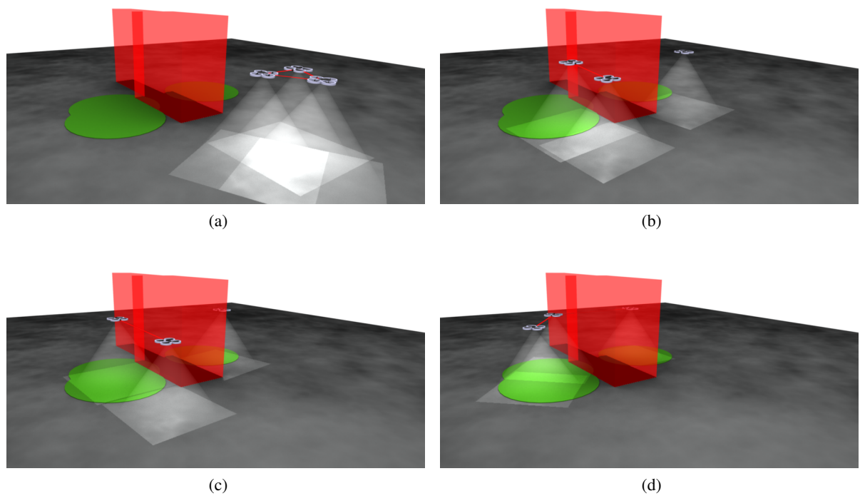
Figure 1.2.: Violation of the relative localization constraints when trajectories are planned after searching the optimal positions. Relative localization constraints are violated in b), c), d). Obstacles are visualized by red colour, AoIs by green colour. Source [23]
