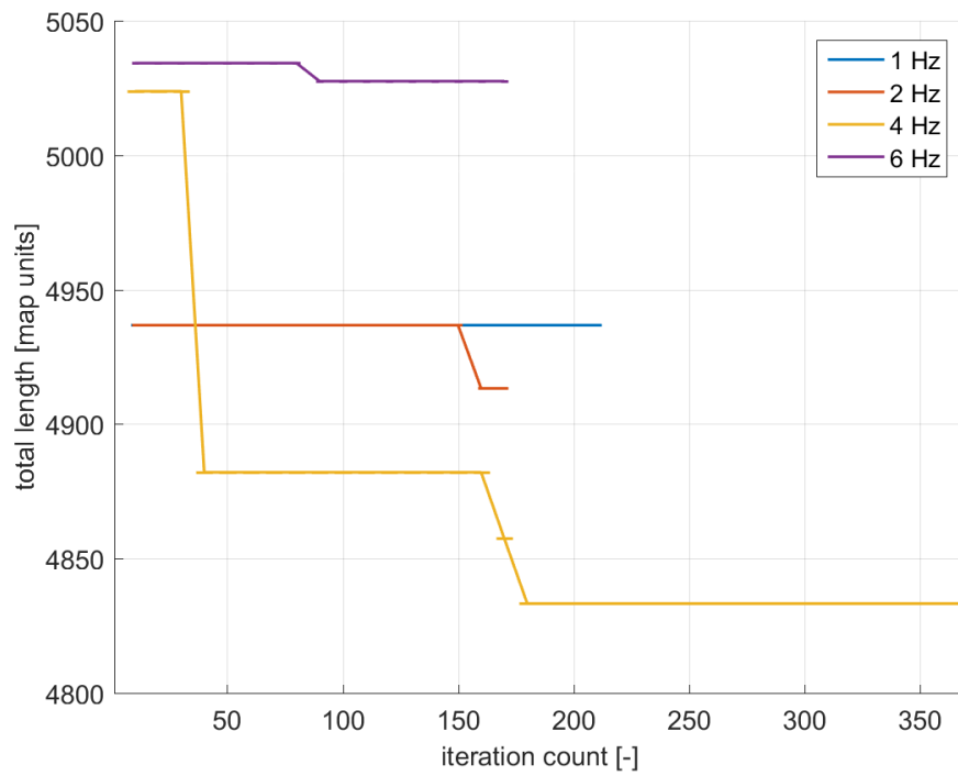
Figure 12.12.: Progress of length of paths during the optimization of trajectory in figure 12.9 for 2 Hz, 4 Hz, 6 Hz. As shown in figure, the optimization got stuck in local optima very soon for frequency 6 Hz.
