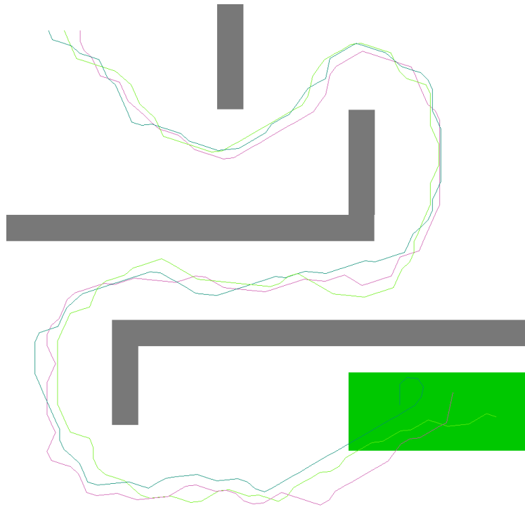
Figure 12.3.: Trajectory before Dubins curves optimization.
