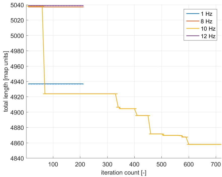
Figure 12.13.: Progress of length of paths during the optimization of trajectory in figure 12.9 for 8 Hz, 10 Hz, 12 Hz.
