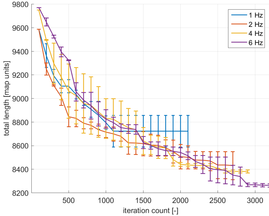
Figure 12.6.: rogress of length of paths during the optimization of trajectory in figure 12.3 for 2 Hz, 4 Hz, 6 Hz
