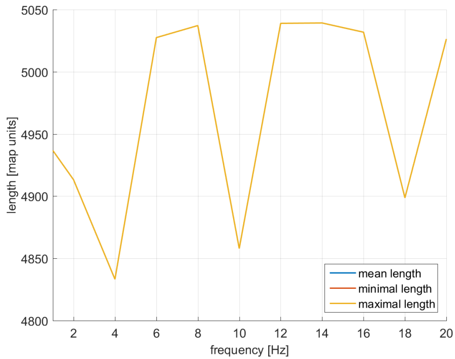
Figure 12.11.: Re-sampling and optimization results graph of experiment 12.2.2. Mean distance, maximal distance and minimal distance are overlapping in this graph. This is caused by zero standard deviation of results at the end of optimization.
