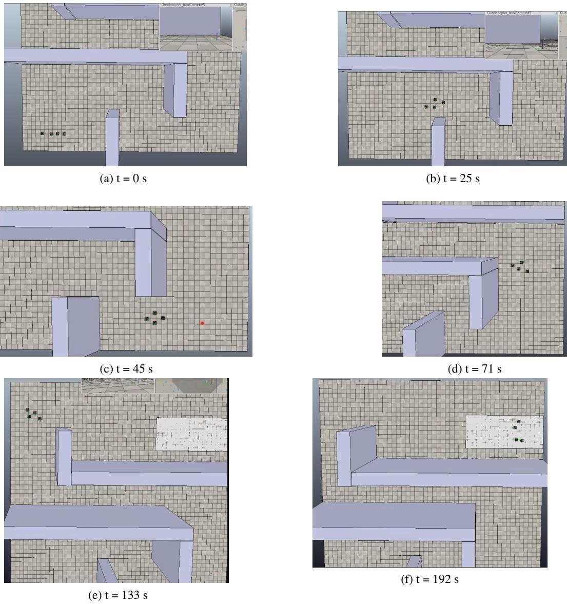
Figure 10.2.: VREP simulation of trajectories in complex map. All UAVs proceeded successfully from the initial position to the AoI, marked with white rectangle. Video with the simulation can be seen in enclosed DVD in the file videos/map0_new.avi . Map used in this simulation is also used in experiments 12.1 and 12.2.1
