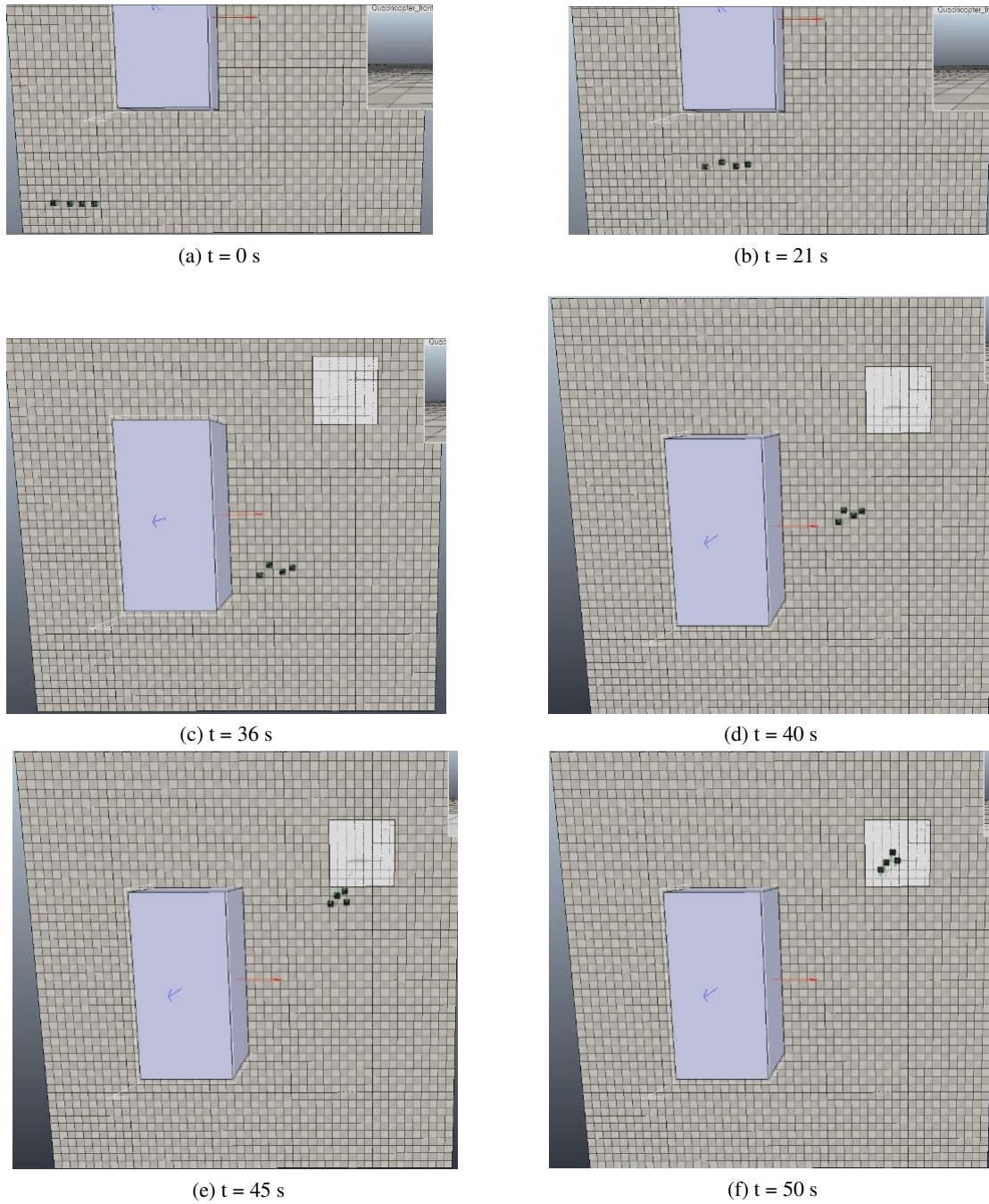
Figure 10.3.: VREP simulation of trajectories in complex map. All UAVs proceeded successfully from the initial position to the AoI, marked with white rectangle. Video with the simulation can be seen in enclosed DVD in the file videos/map3_new.avi. Map used in this simulation is also used in experiments 12.1 and 12.2.1
