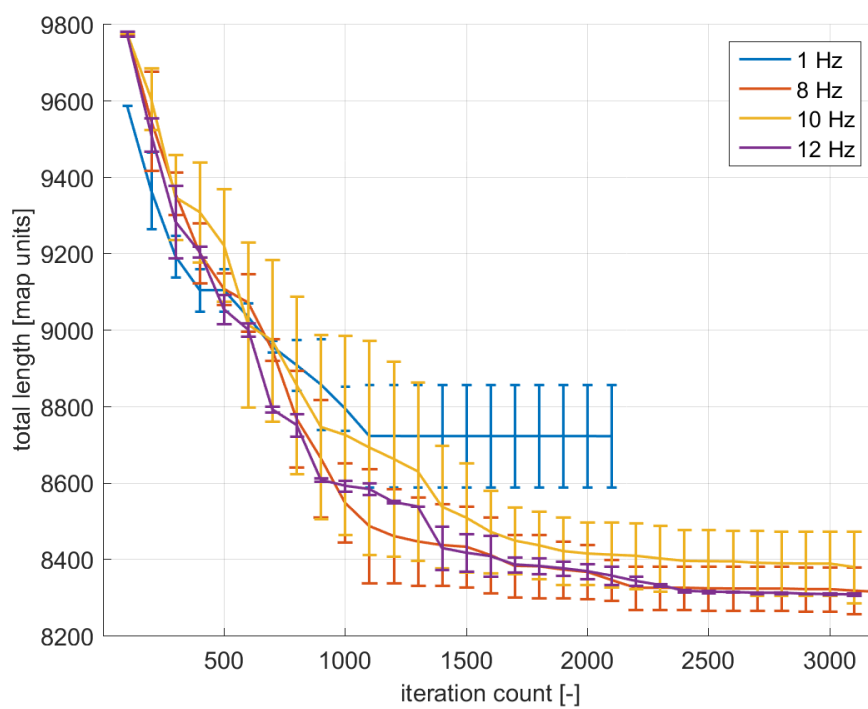
Figure 12.7.: Progress of length of paths during the optimization of trajectory in figure 12.3 for 8 Hz, 10 Hz, 12 Hz
