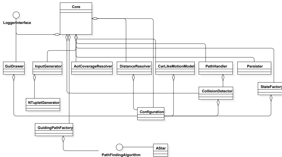
Figure 11.1.: Dependency diagram
