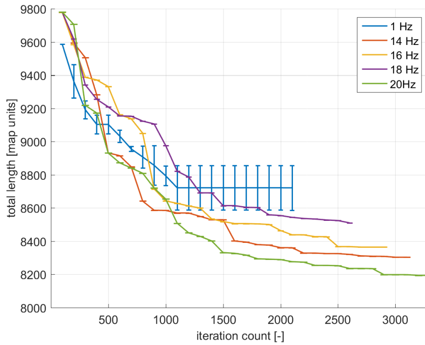
Figure 12.8.: Progress of length of paths during the optimization of trajectory in figure 12.3 for 14 Hz, 16 Hz, 18 Hz, 20 Hz
