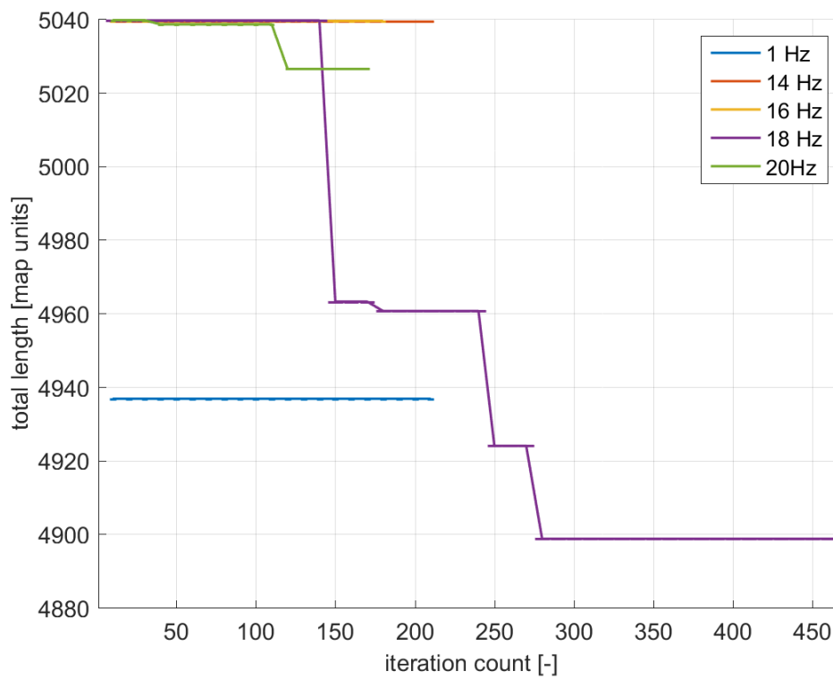
Figure 12.14.: Progress of length of paths during the optimization of trajectory in figure 12.9 for 14 Hz, 16 Hz, 18 Hz, 20 Hz.
