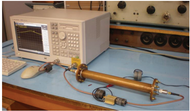
Fig. 4. Experimental setup for the measurement of resistance.
