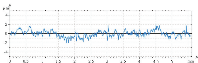
Fig. 9. Typical roughness of surface of measured rods. Roughness was measured along the axis of the rod.
