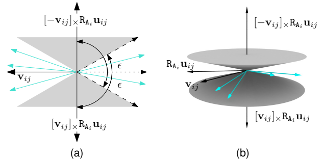
Figure 2. (a) Geometric interpretation of the \epsilon -epipolar constraint with parameter \epsilon imposed by the correspondence \mathbf{u}_{ij} \leftrightarrow \mathbf{v}_{ij} on the position of \mathbf{t}_{A_i} . The cyan vectors show examples of the admissible configurations of \mathbf{t}_{A_i} . (b) 3D view of the same.
