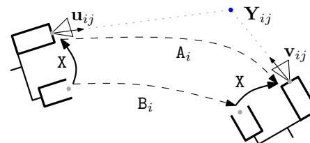
Figure 1. A gripper-camera rig motion.
