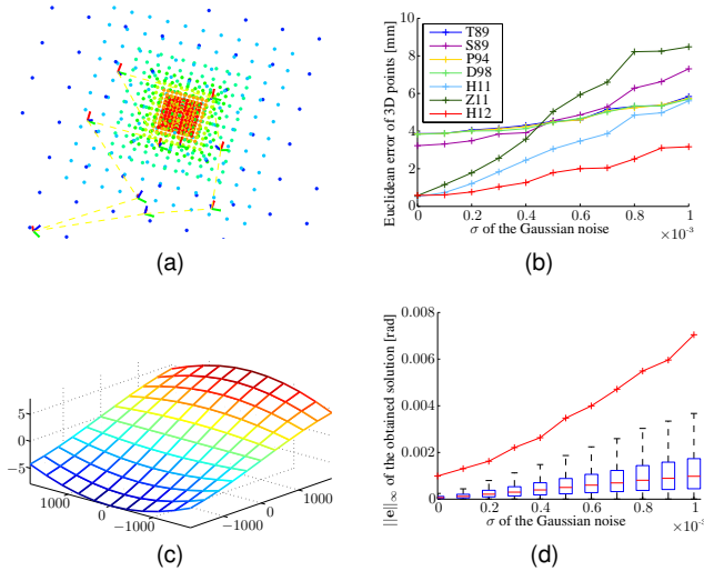
Figure 5. Planar experiment. (a) Camera positions in the experiment, different colors encode positions of the 3D points at different FOV levels. (b) Comparison of the proposed method with previous methods using Euclidean distance measure. (c) Grid deformation (not in scale). (d) The maximum (red line) and median (boxes) residual error of the obtained solutions for the various values of \sigma .
