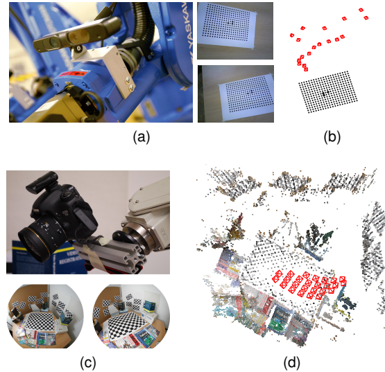
Figure 6. Real data experiment. (a–b) Motoman MA1400. Close up of the camera-gripper rig, sample images from the sequence; Camera poses reconstruction (c–d) Mitsubishi MELFA-RV-6S. Close up of the camera-gripper rig, sample images from the sequence; Model resulting from SfM, cameras are denoted by red pyramids.
