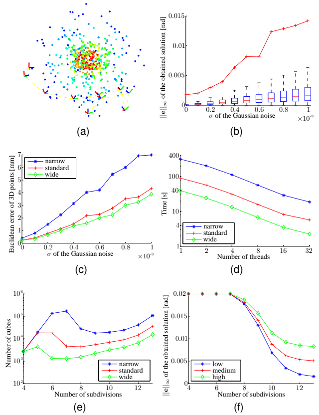
Figure 4. Ball experiment. (a) Camera positions in the experiment, different colors encode positions of the 3D points at different FOV levels. (b) The maximum residual error of the obtained solutions for the various values of \sigma (red line) and the distribution of the measured errors over all correspondences (boxes). (c) The mean Euclidean distance between the 3D points transformed to the gripper’s coordinate systems using ground truth X and the 3D points transformed to the gripper’s coordinate systems using the estimated X . The 8 FOV levels were merged into three groups. (d) Loglog plot of the computational time as a function of the number of threads. (e) The mean number of remaining cubes plotted against the number of subdivision phases. Note that the computation starts after the fourth subdivision. (f) The mean residual error at the beginning of the respective subdivision phase. Different noise levels were clustered into three groups.
