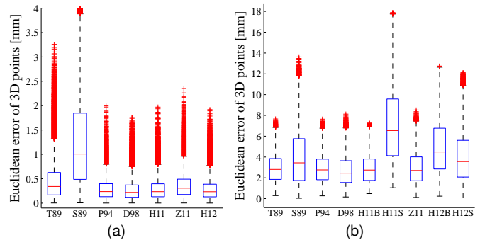
Figure 7. Real data experiment error. (a) Motoman MA1400 (b) Mitsubishi MELFA-RV-6S.
