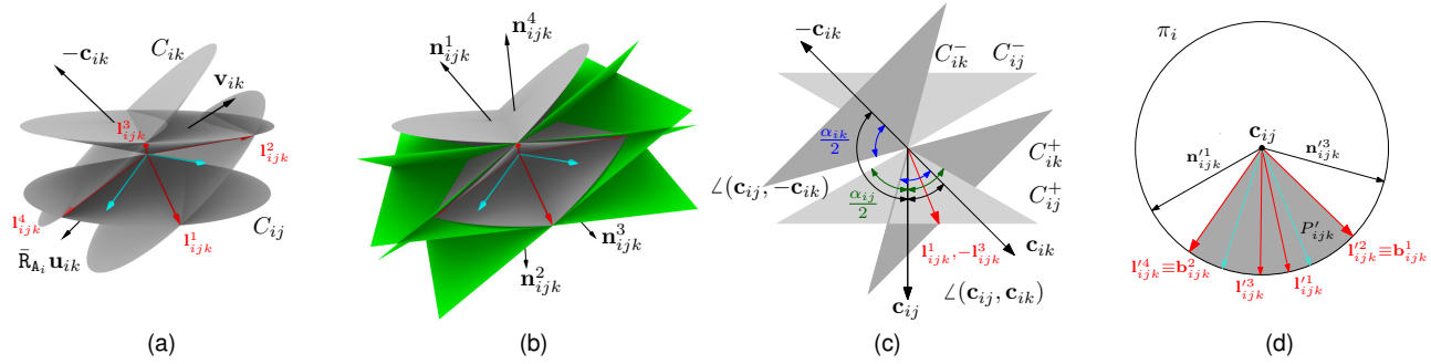
Figure 3. (a) If the apertures \alpha_j, \alpha_k are sufficiently large, cones C_{ij} and C_{ik} intersect in up to four lines l^1_{ijk}, l^2_{ijk}, l^3_{ijk}, l^4_{ijk} . (b) The linear constraints imposed by correspondences u_{ij} \leftrightarrow v_{ij}, u_{ik} \leftrightarrow v_{ik} are determined by the normals n^1_{ijk}, n^2_{ijk}, n^3_{ijk}, n^4_{ijk} . (c) Since Inequality 2 holds, the nappes C_{ij}^+, C_{ik}^+ intersect in l^1_{ijk} and -l^3_{ijk} . However, Inequality 3 does not hold and the cones C_{ij}, C_{ik} do not form the pyramid P_{ijk} . (d) The projection of the pyramid P_{ijk} into the plane \pi_i determined the boundary vectors b^1_{ijk}, b^2_{ijk} (a 2D projection of the situation in (b)).
