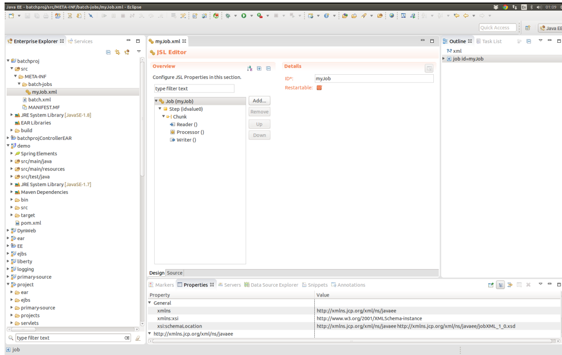
Figure 3.2. Tree-form XML editor in WebSphere Developer Tools
