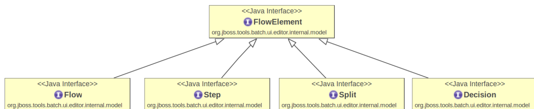
Figure 4.2. Part of initial Sapphire model — flow elements
