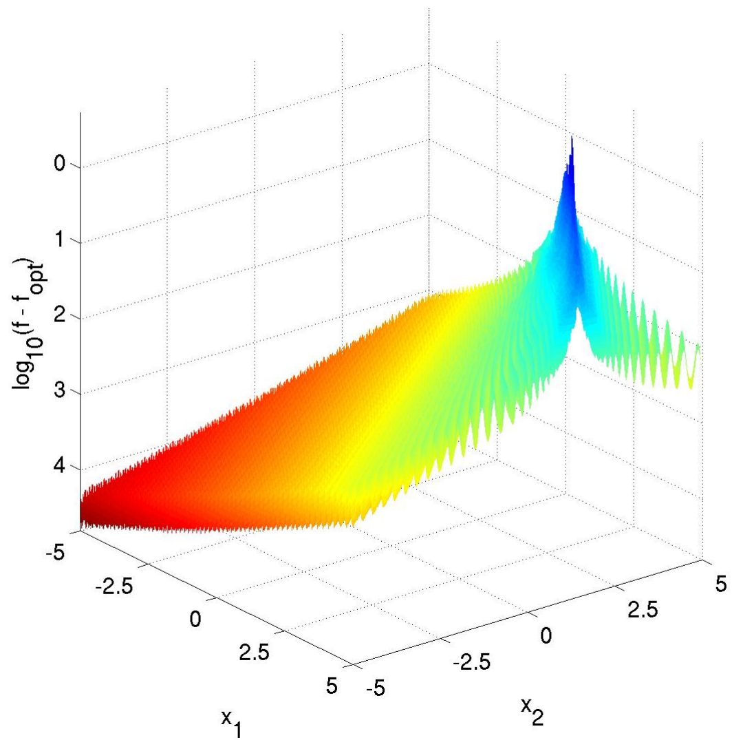
Obrázek A.18: Funkce 18 (Schaffers F7 Function, moderately ill-conditioned)
