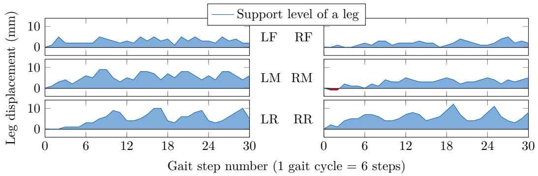
Figure 6.4. Support level of all legs while walking on a flat ground with S_0 = 40 mm.
