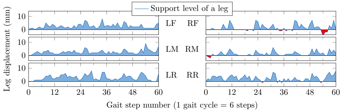
Figure 6.15. Support level of all legs while climbing stairs with S_0 = 30 mm.
