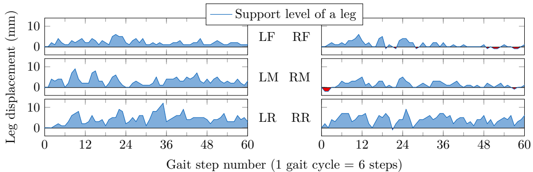
Figure 6.10. Support level of all legs while walking on a 10^\circ slope with S_0 = 60 mm.
