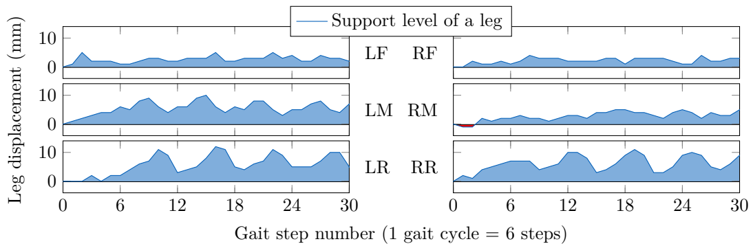
Figure 6.5. Support level of all legs while walking on a flat ground with S_0 = 50 mm.
