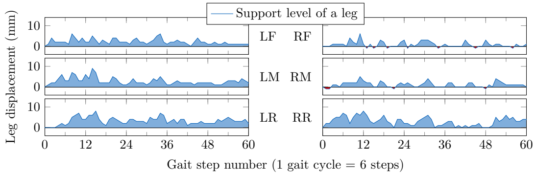
Figure 6.7. Support level of all legs while walking on a 10^\circ slope with S_0 = 30 mm.
