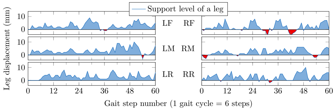
Figure 6.16. Support level of all legs while climbing stairs with S_0 = 40 mm.
