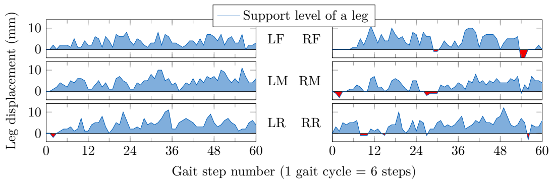
Figure 6.18. Support level of all legs while climbing stairs with S_0 = 60 mm.
