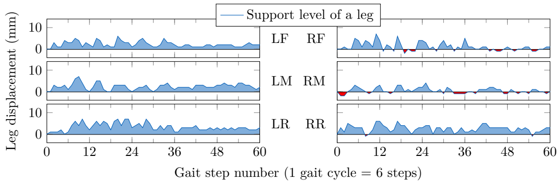
Figure 6.12. Support level of all legs while walking on a 20^\circ slope with S_0 = 40 mm.
