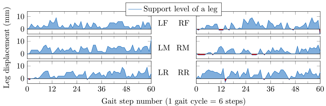
Figure 6.17. Support level of all legs while climbing stairs with S_0 = 50 mm.
