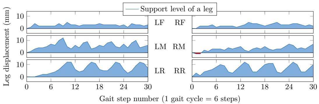
Figure 6.6. Support level of all legs while walking on a flat ground with S_0 = 60 mm.
