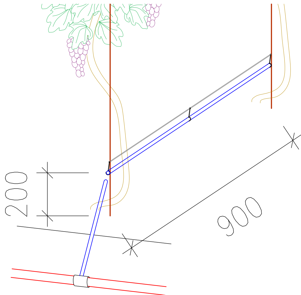
DETAIL (M 1:10)
