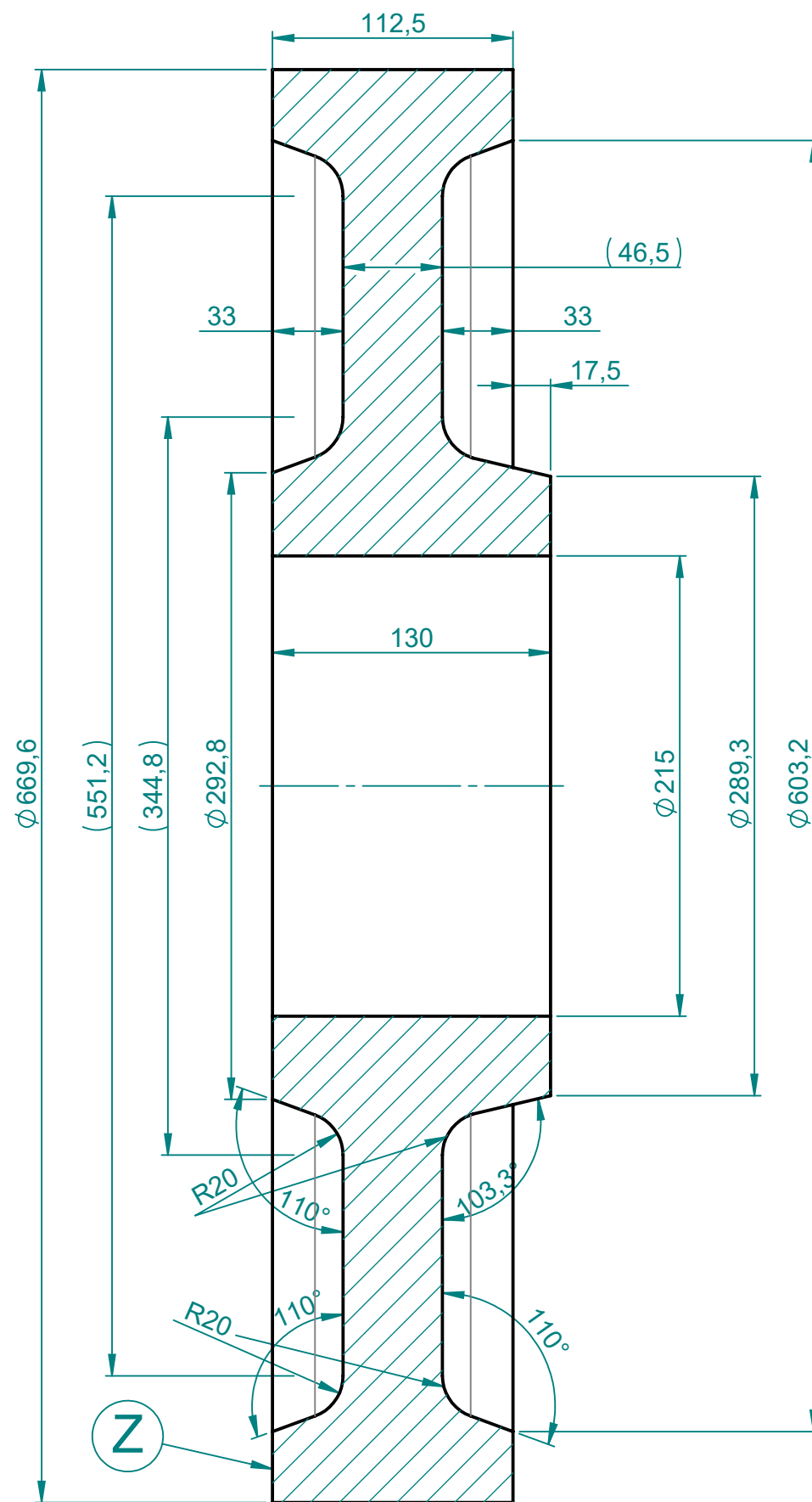
Tvar vykovku Shape of forging
