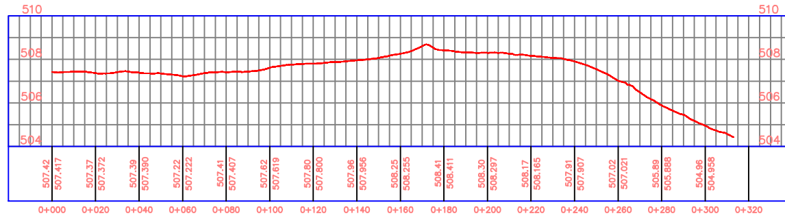
Stoka E PROFILE
