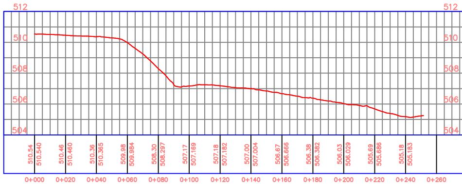
Stoka D – nová PROFILE
