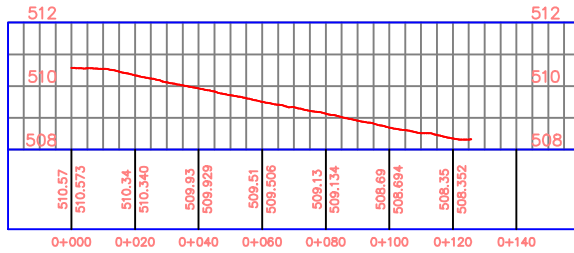
Stoka D – nová PROFILE
