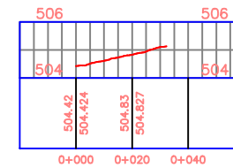
Stoka D-1 PROFILE
