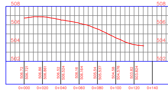
Stoka E PROFILE
