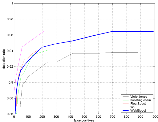
Fig. 1. ROC curve comparison of the WaldBoost algorithm with the state-of-the-art methods.
