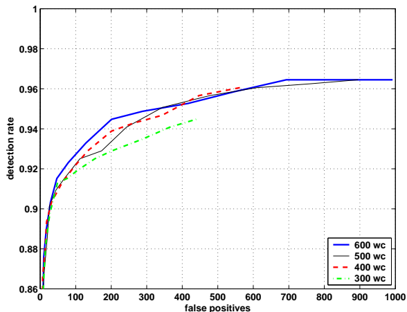
Fig. 2. The effect of reducing the number of weak classifiers in WaldBoost classifier on the detection rate.
