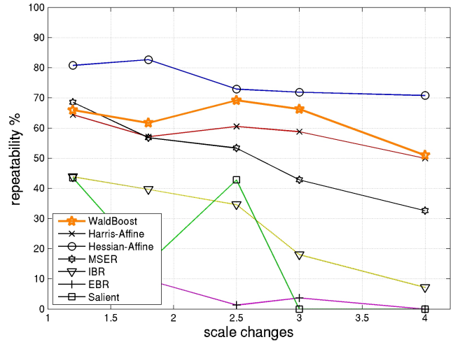
Fig. 5. Repeatability score of the WaldBoost detector for Bark sequence (overlap 40%, norm. size = 30 pixels).
