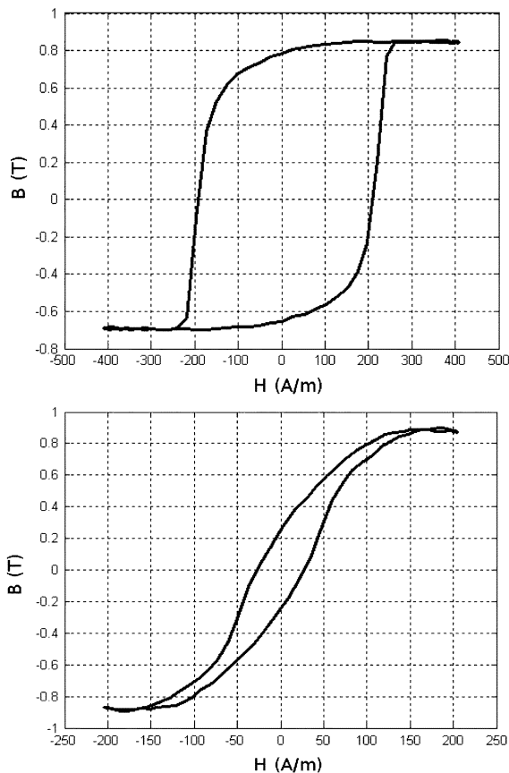
Fig. 1. B(T) - H(A/m) loops in longitudinal (a) and circumferential (b) direction.
