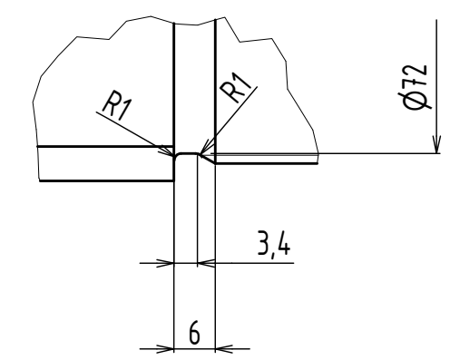
F (1:1)
