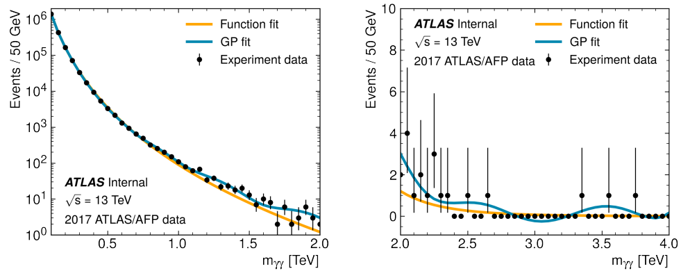
Figure 5.10: Comparison of background modelling results on wide mass range from 100 GeV to 4000 GeV.
