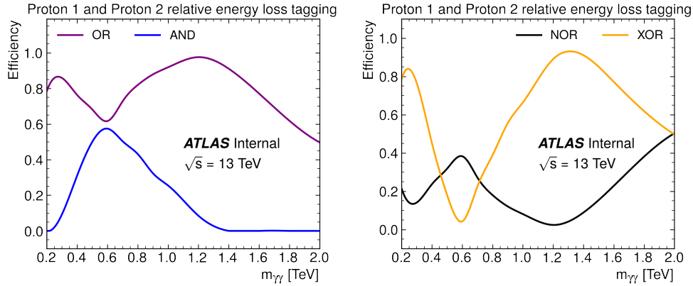
Figure 4.6: Proton tagging probabilities in axion-like particle production process based on scattered diphoton invariant mass.
