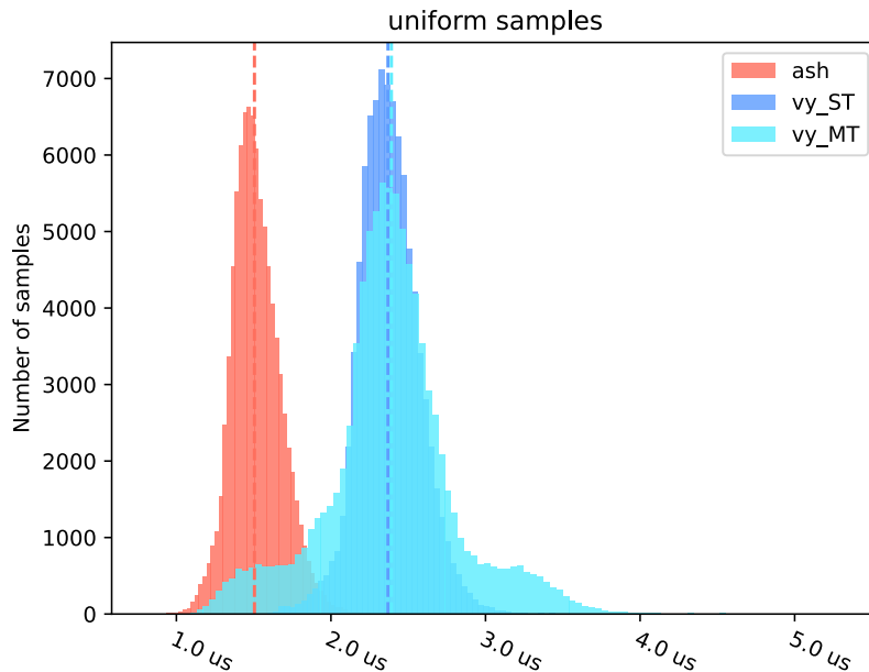
Figure 5.5: Histogram of uniform stage of the benchmarks ( n = 99000 ). It is clear that ash is faster than both single- and multi-threaded Vulkanes. However, the overhead is constant.
