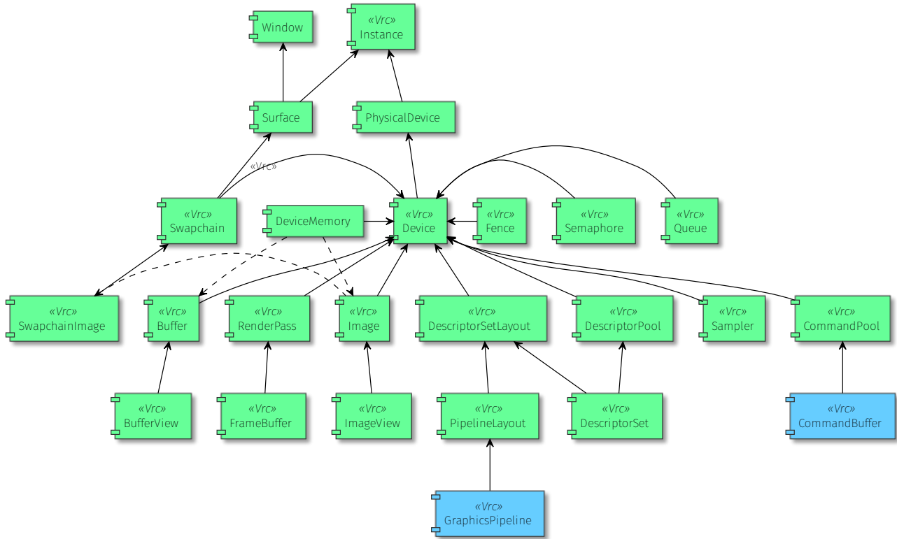
Figure 3.1: Object Dependency Graph of Vulkan
