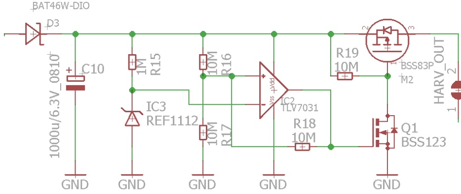
Fig. 2: Schematic of the harvester circuit
