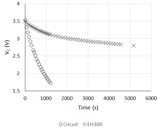
Fig. 3: Measurement of the voltage drop on the storage capacitor during the time caused by the leakage currents
