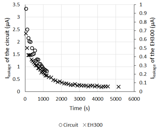
Fig. 4: Leakage currents of the devices calculated from the voltage drop
