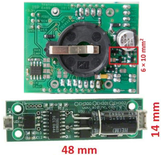
Fig. 6: Comparison of the harvesting circuit footprint (top) with the harvester EH300 (bottom)
