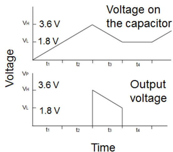
Fig. 1: Operating cycle of the harvester EH300 [2]
