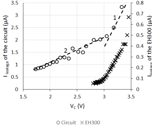
Fig. 5: Comparison of the presented circuit and harvester EH300 leakage currents versus the actual voltage on the capacitor
