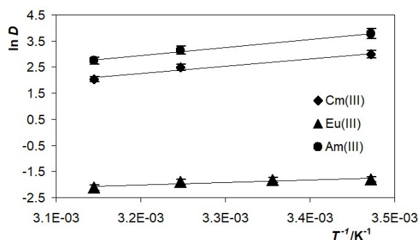
Figure 4. Dependency of \ln D_{\text{Am,Cm,Eu}} \pm \sigma on 1/T used for the calculation of the reaction enthalpy, \Delta H , and entropy, \Delta S , by means of Equation (12)
