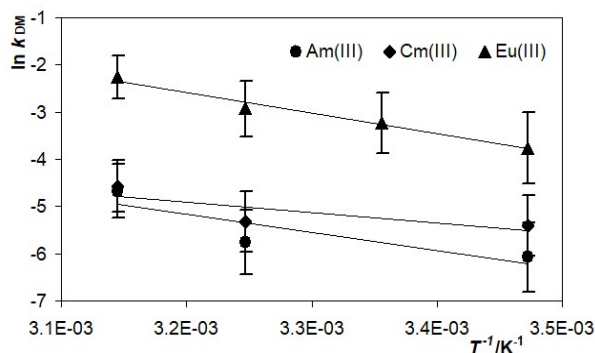
Figure 5. Dependence of \ln(k_{DM})_{Am,Cm,Eu} \pm \sigma on 1/T used for the calculation of the apparent activation energy, E_a , and the frequency factor, k_0 , by means of the Arrhenius equation (8)
