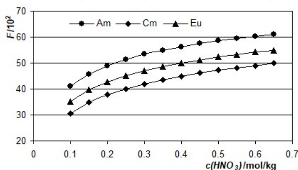
Figure 2. Molar fractions, F/10^2 , of the given complexes \text{MNO}_3^{2+} as a function of \text{NO}_3^- concentration [\text{mol}\cdot\text{kg}^{-1}] .
