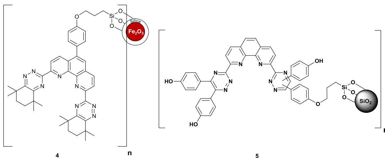
Fig. 2 Structural formulae of CyMe 4 -BTPhen-functionalized SiO 2 -coated MNP 4 and tetra(4-hydroxyphenyl)-BTPhen-functionalized SiO 2 gel 5 .
