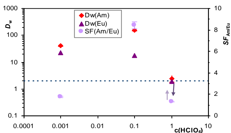
Fig. 5 Extraction of Am(III) and Eu(III) by CyMe 4 -BTPhen-functionalized SiO 2 -coated MNPs 4 as a function of HClO 4 concentration. Mass of sorbent: approximately 18 mg, phase volume: 0.6 mL, V/m ratio: ~ 33 mL g -1 .
