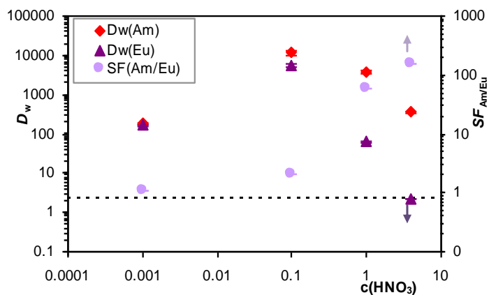
Fig. 3 Extraction of Am(III) and Eu(III) by CyMe_4 -BTPhen-functionalized SiO_2 gel 8 as a function of HNO_3 concentration. Mass of sorbent: approximately 16 mg, phase volume: 1 mL, V/m ratio: \sim 60 \text{ mL g}^{-1} .
