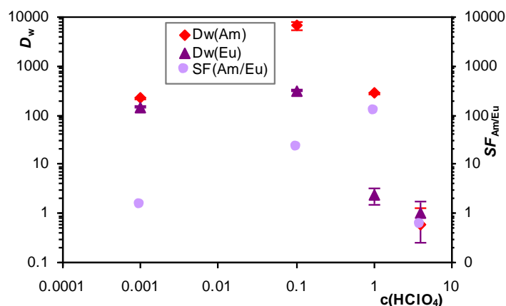
Fig. 4 Extraction of Am(III) and Eu(III) by CyMe_4 -BTPhen-functionalized SiO_2 gel 8 as a function of HClO_4 concentration. Mass of sorbent: approximately 15 mg, phase volume: 0.6 mL, V/m ratio: \sim 40 \text{ mL g}^{-1} .
