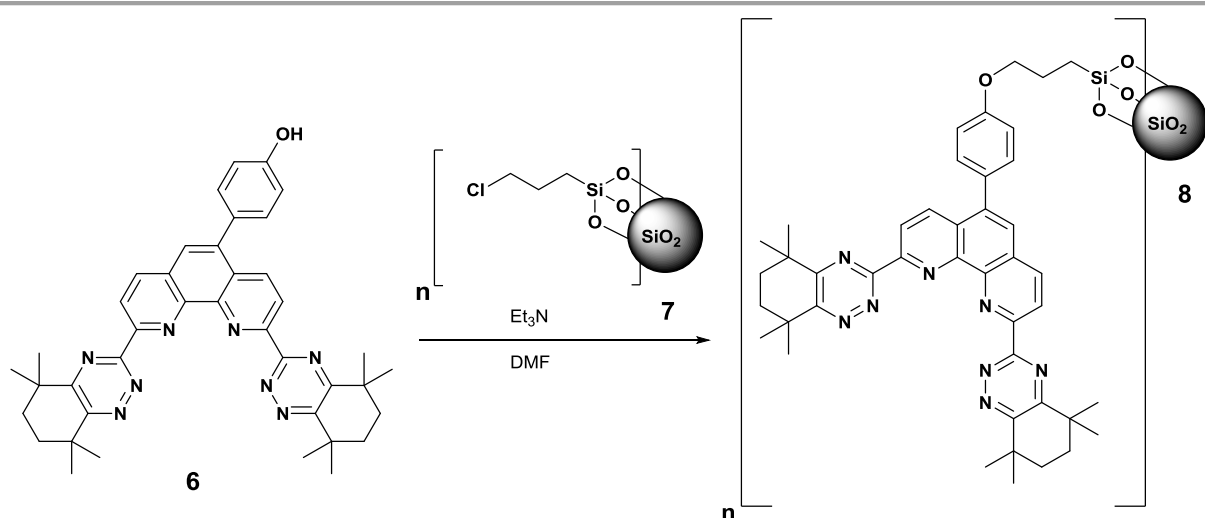
Scheme 1 Immobilization of (4-hydroxyphenyl) functionalized CyMe 4 -BTPhen 6 on silica gel.
