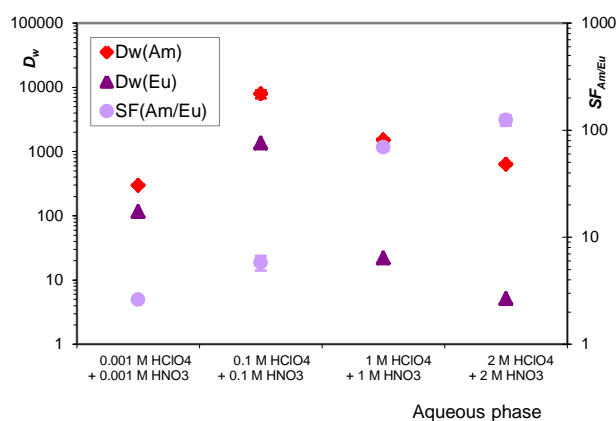
Fig. 6 Extraction of Am(III) and Eu(III) by CyMe 4 -BTPhen-functionalized SiO 2 -coated MNPs 4 as a function of HClO 4 /HNO 3 concentration. Mass of sorbent: approximately 15 mg, phase volume: 0.6 mL, V/m ratio: ~ 40 mL g -1 .
