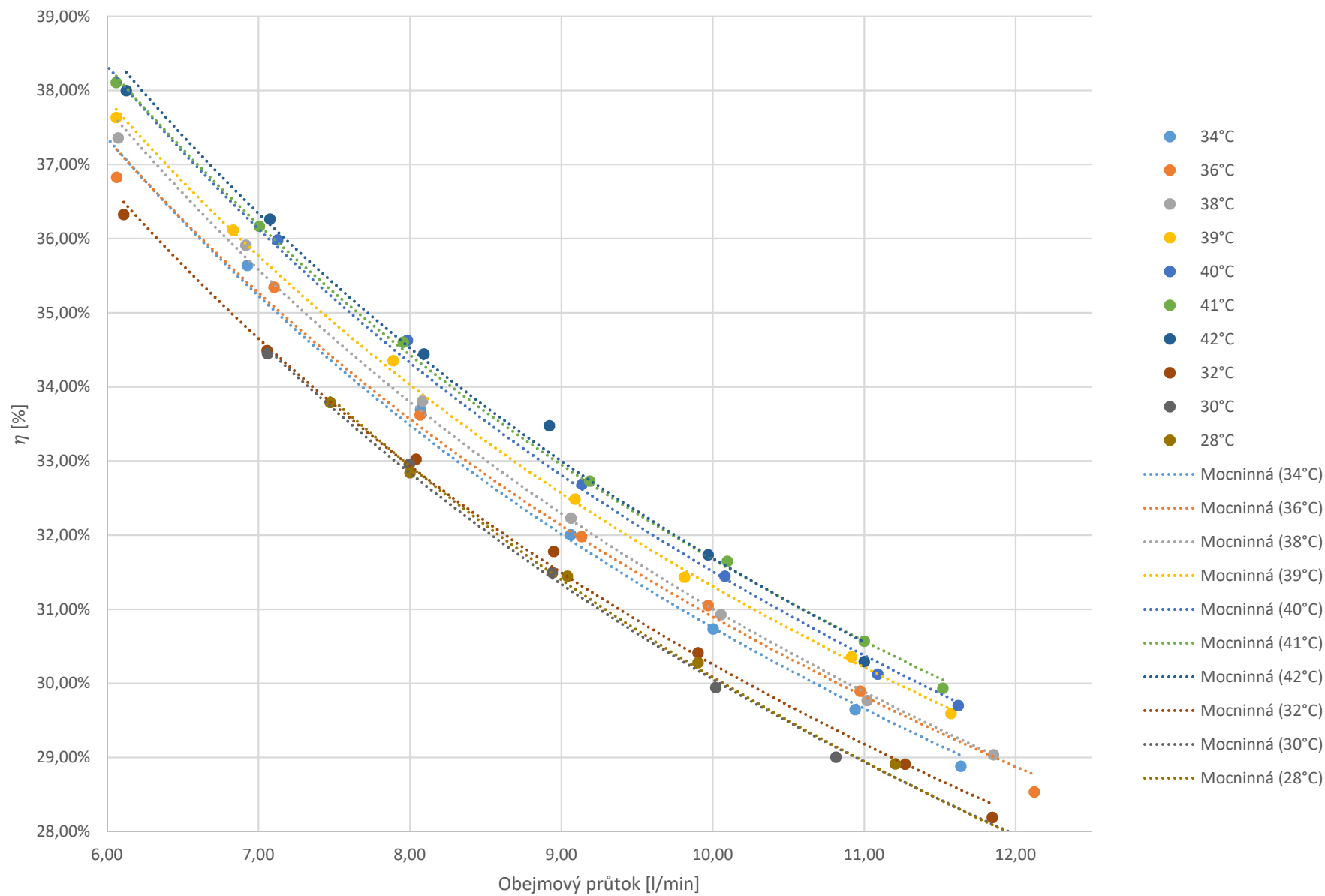
Tmix 34,36,38,39,40,41,42 °C
