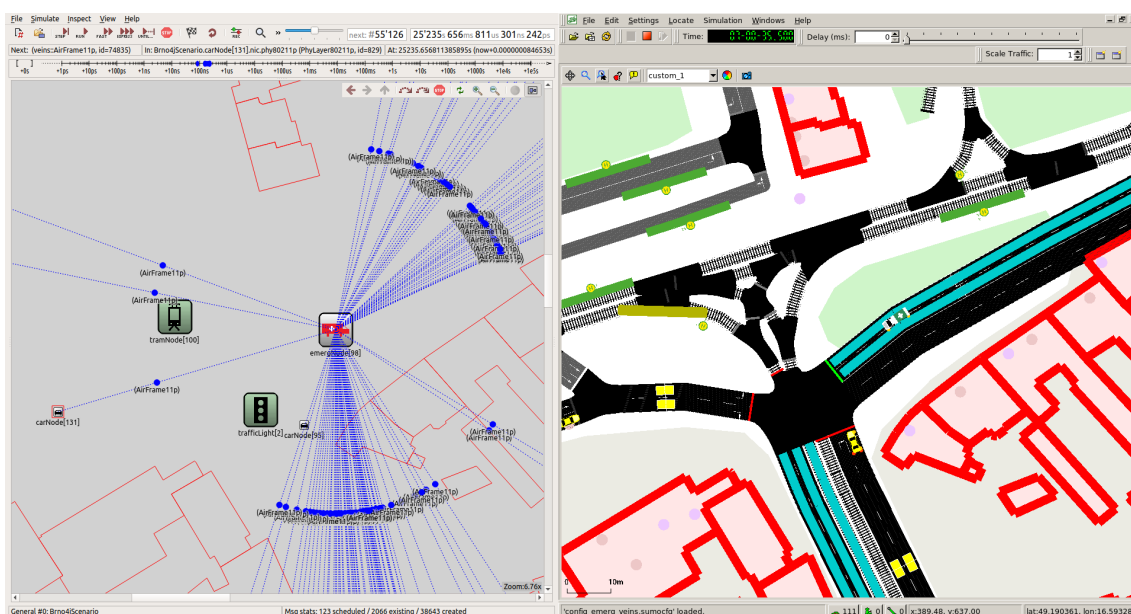
Figure 4.11: Running simulation of the queue discharge based method in the scenario of Brno. On the left, the simulation of V2X communication in GUI of OMNeT++. On the right, the mobility simulation in SUMO-GUI. They are coupled by sumo_launchd.py .
