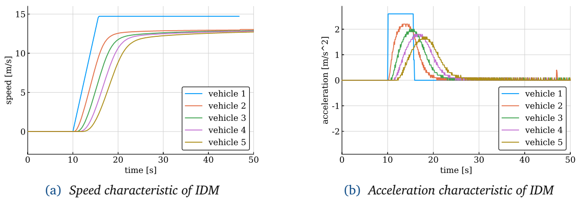
Figure 2.2: Five simulated vehicles in a queue governed by IDM starts off at time 10.
