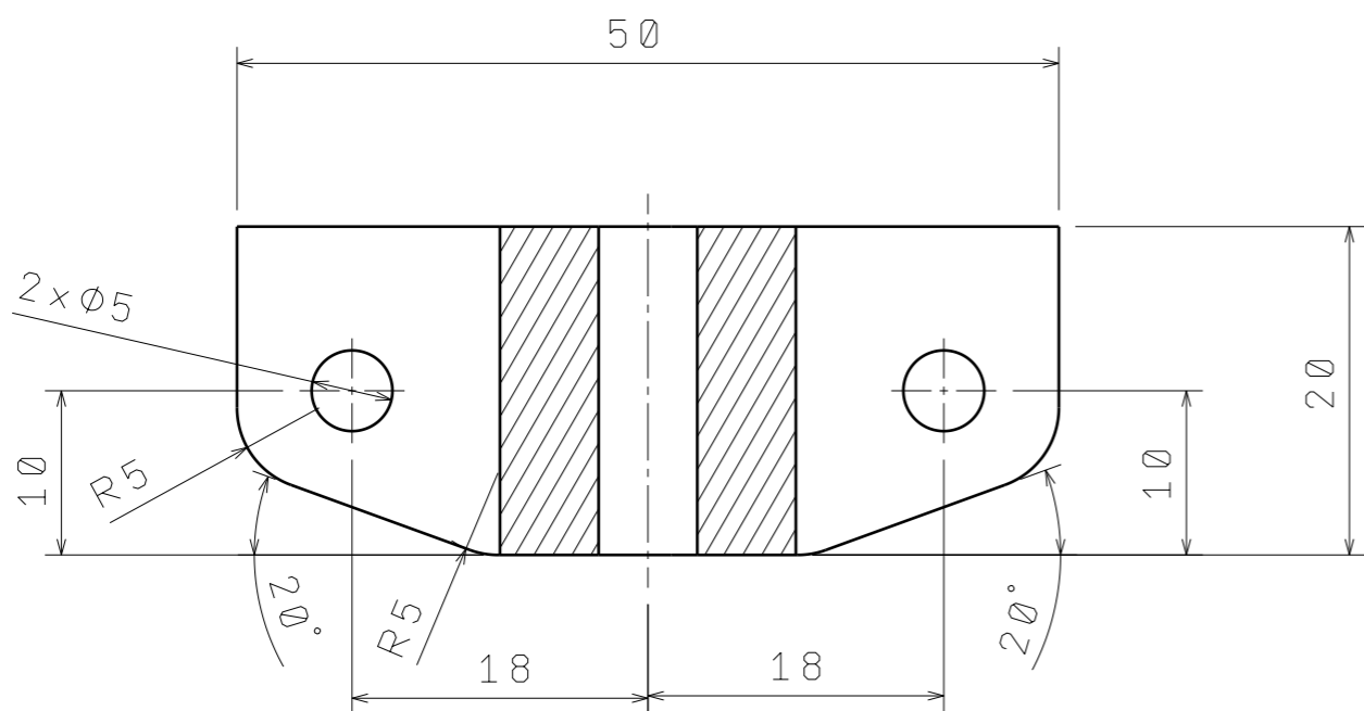
Section view B-B Scale: 2:1
