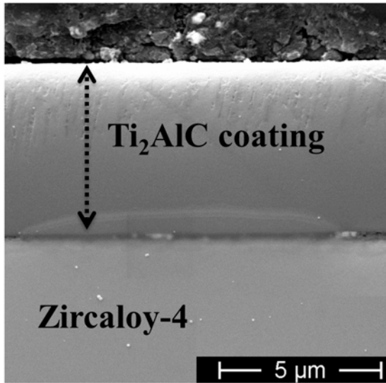
FIGURE 4. SEM images of cross-section view of \text{Ti}_2\text{AlC} coating on Zry-4.
