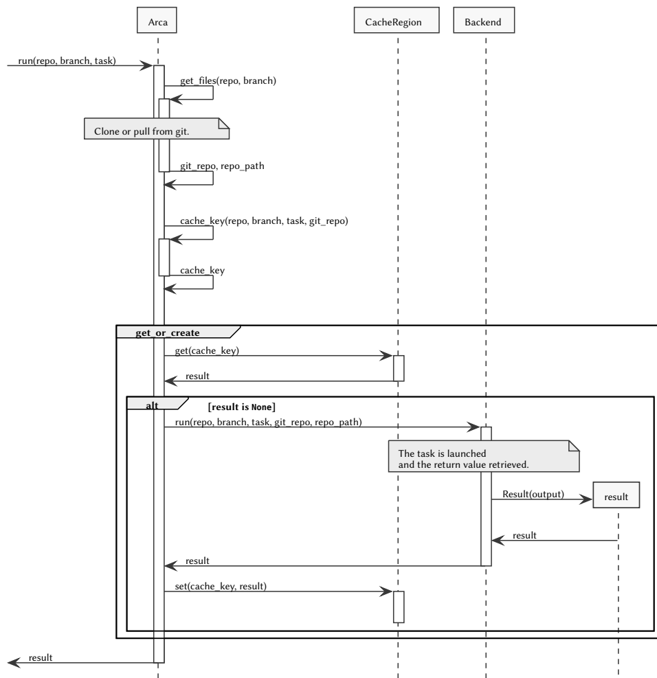
Figure 3.2: UML sequence diagram of the Arca run method
