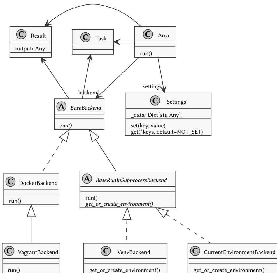
Figure 3.1: UML class diagram of classes used in Arca
