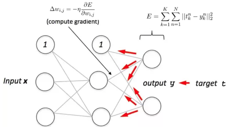
Figure 2.5: Backpropagation and weight update. [28]
