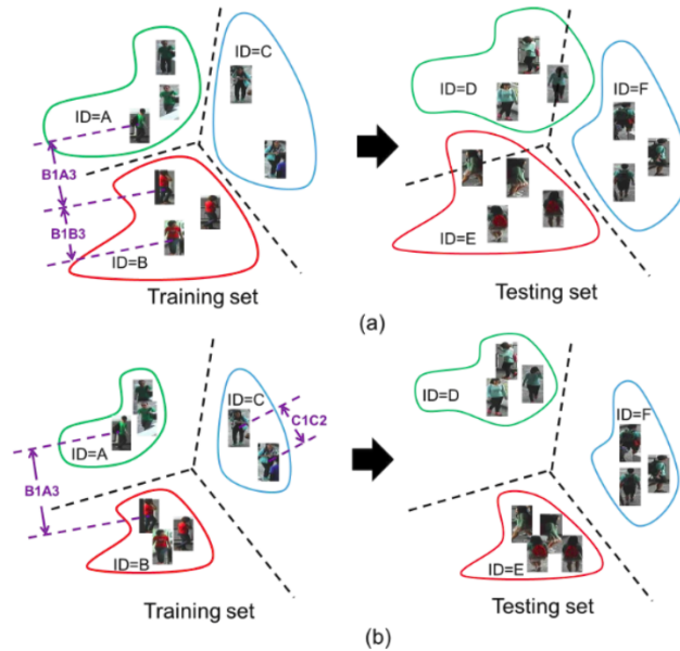
Figure 3.1: (a) Visualization of the low generalization with triplet loss function (b) Visualization of the better generalization with quadruplet loss function [5]
