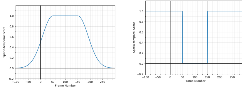
(b) : Function for calculation spatio-temporal score for cameras far away.
