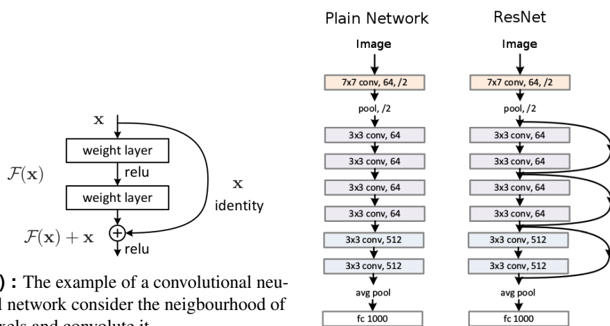
(b) : On the left image is the plain neural network and on the right side is the ResNet. There is only one difference - the "shortcuts".
