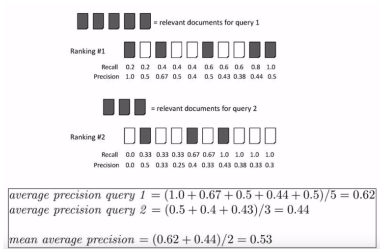
Figure 2.13: Example of calculation of the Mean Average Precision (mAP) [41]
