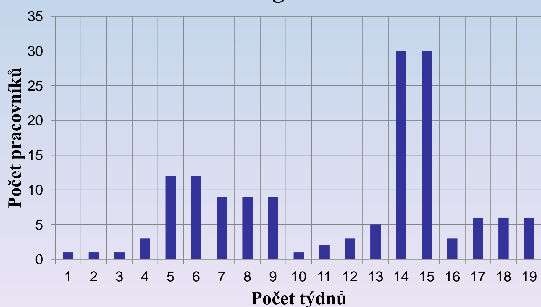
Histogram
