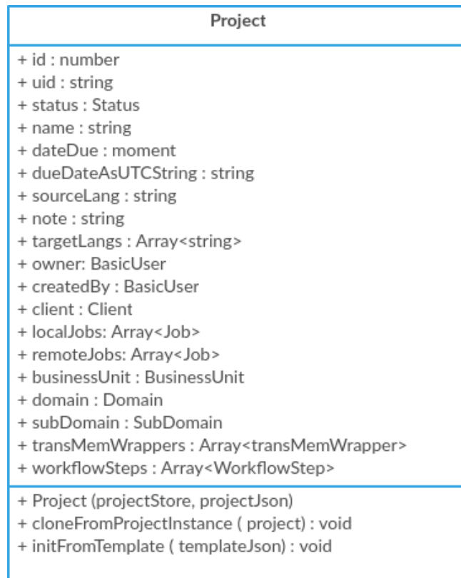
Figure 3.8: Project class
