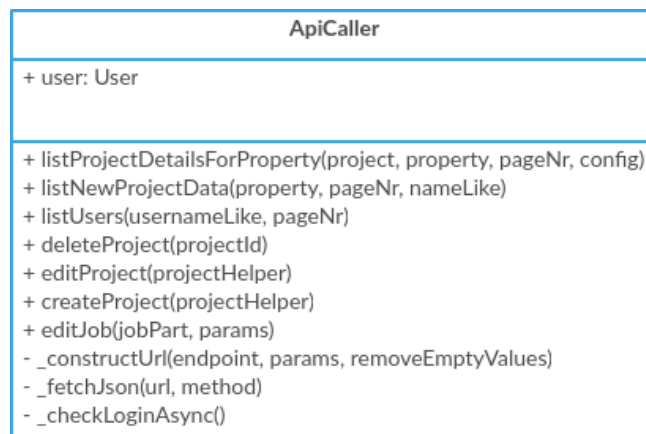
Figure 3.7: ApiCaller class
