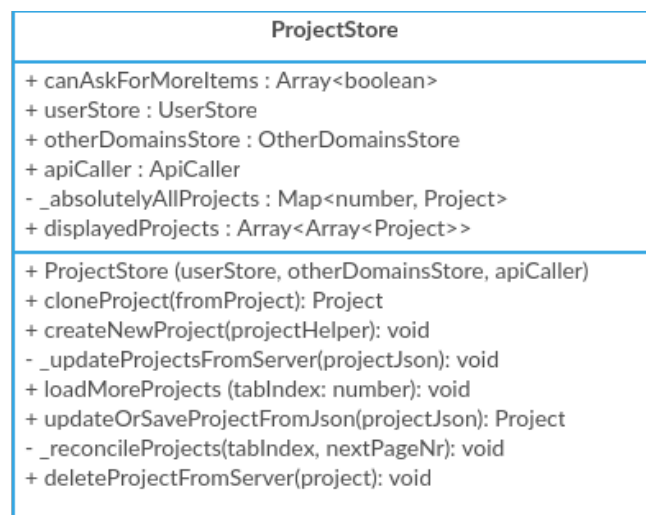
Figure 3.9: ProjectStore class
