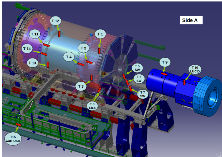
Figure 1.1: TPX detectors installed within the ATLAS machine at CERN.
