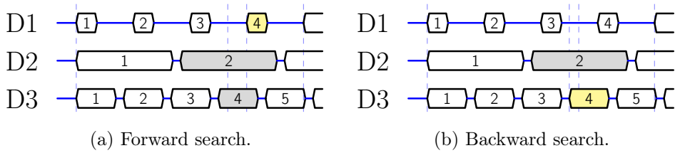
Figure 3.2: Time diagram of frame search illustrating behavioral differences between search modes. Individual blocks correspond with periods of detector acquisition. Emphasized blocks are returned as the search result (yellow marks the master frame). Dashed lines mark the first minute of footage, the search time parameter and the start time of the master frame.
