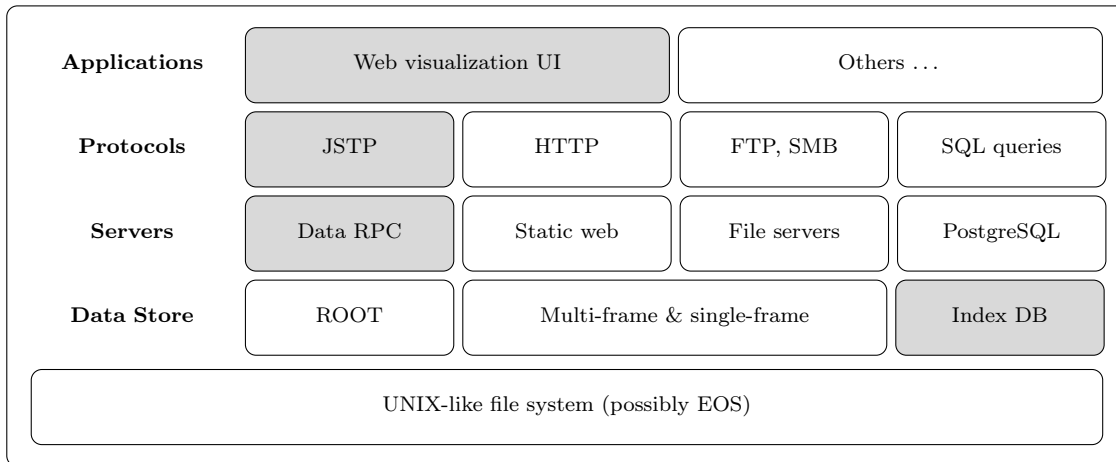
Figure 3.1: A multi-layered system. Proprietary components are emphasized by gray color.
