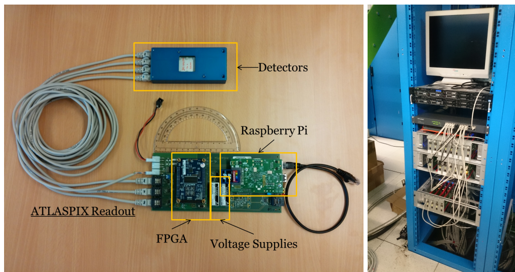
Figure 1.2: The ATLASPIX read-out interface installed at CERN.
