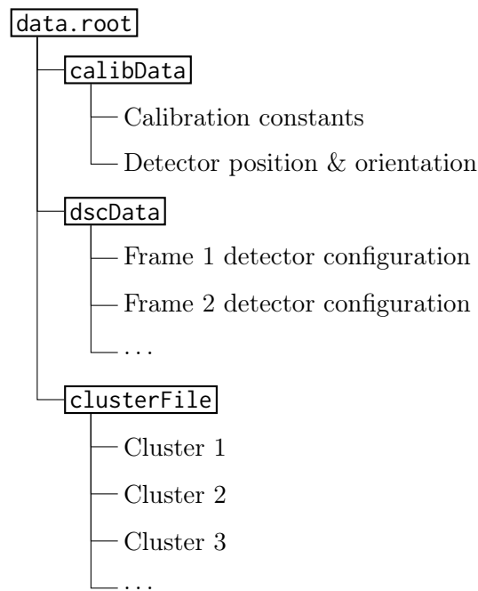
Figure 1.4: Structure of a ROOT file containing TPX footage.
