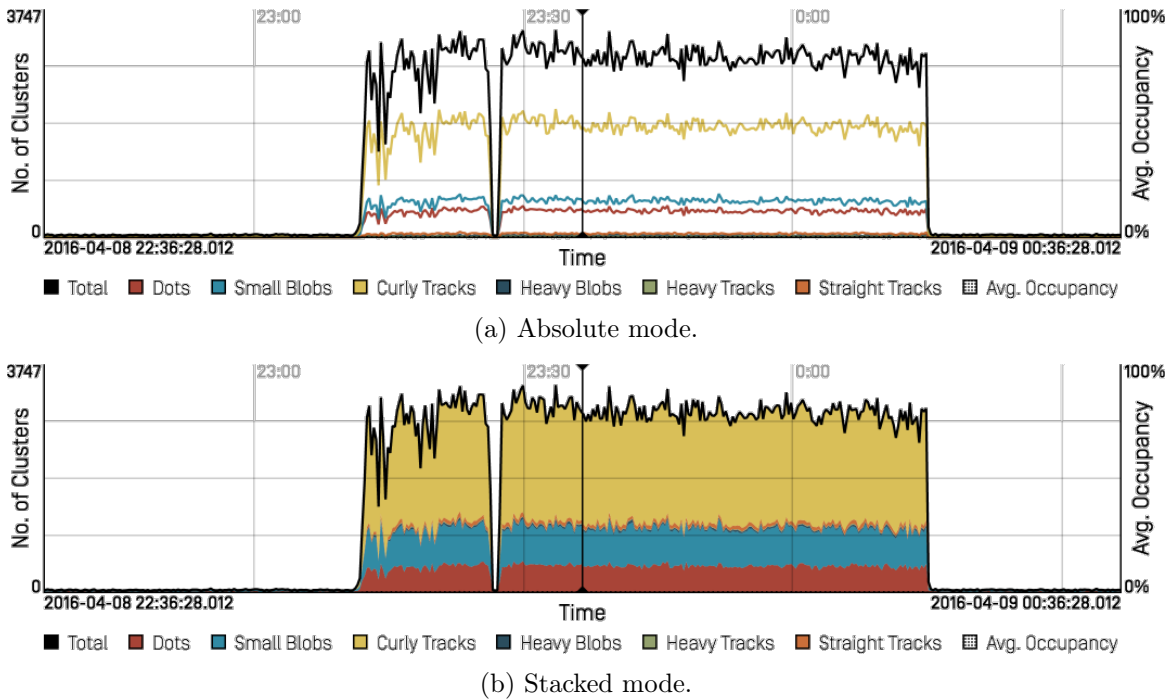
Figure 4.4: Example of the same overview chart rendered in different modes.
