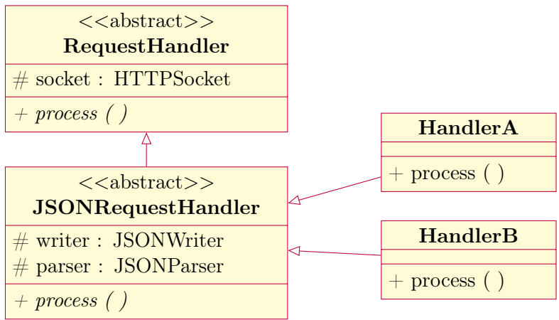
Figure 4.2: UML diagram illustrating the inheritance of request handler objects.
