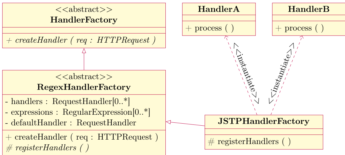
Figure 4.1: UML diagram illustrating the abstract factory design pattern applied in the context of request handler instantiation.
