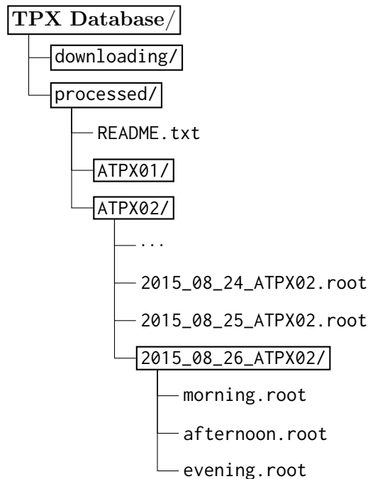
Figure 2.1: Example of the database file system structure.
