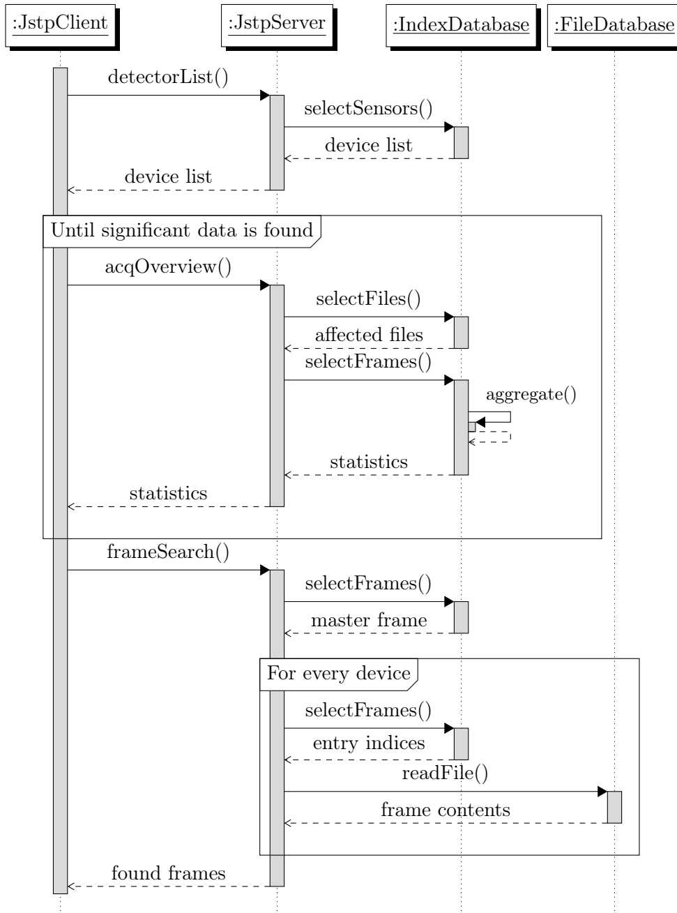
Figure 3.3: UML diagram depicting expected interactions between JSTP client and server, hinting levels of processing complexity at server-side.
