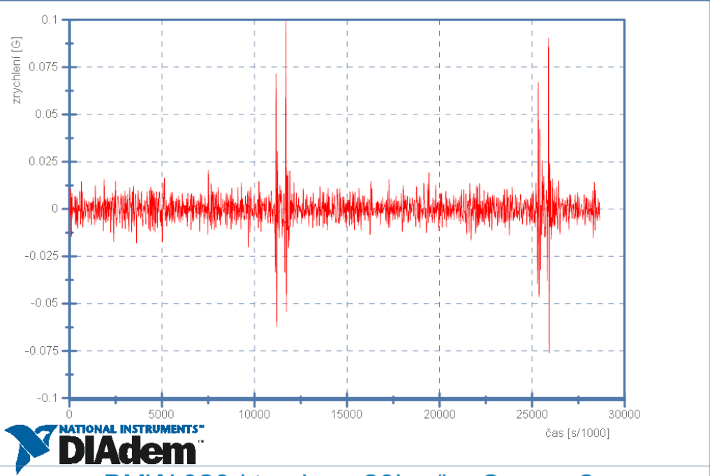
BMW 320d touring - 20km/h - Senzor 2
