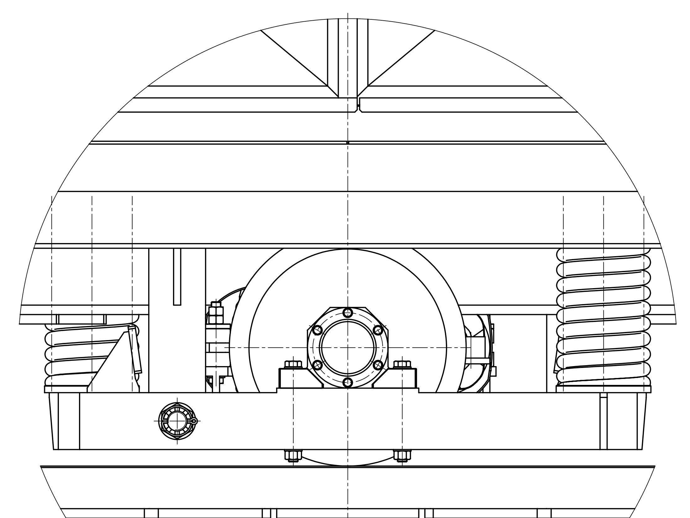
B (1:5)
