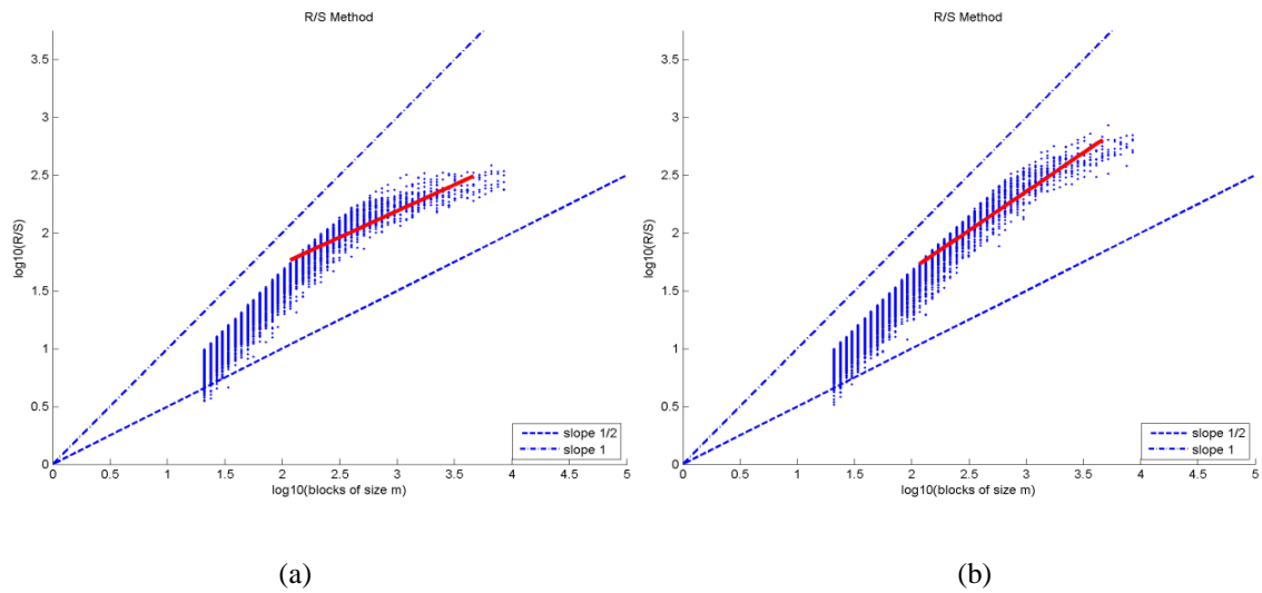
Figure 8.1: R/S estimation of the Hurst exponent, channel Fp1, for (a) quiet and (b) active sleep stage.
