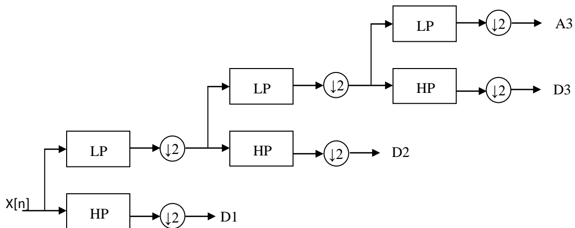
Figure 4.3: Third level wavelet decomposition of a signal. The coefficients D_1 , D_2 , D_3 and A_3 represent the frequency content of the original signal within the bands fs/4 - fs/2 , fs/8 - fs/4 , fs/16 - fs/8 and <fs/16 , respectively, where fs is the sampling frequency of the original signal x[n] .
