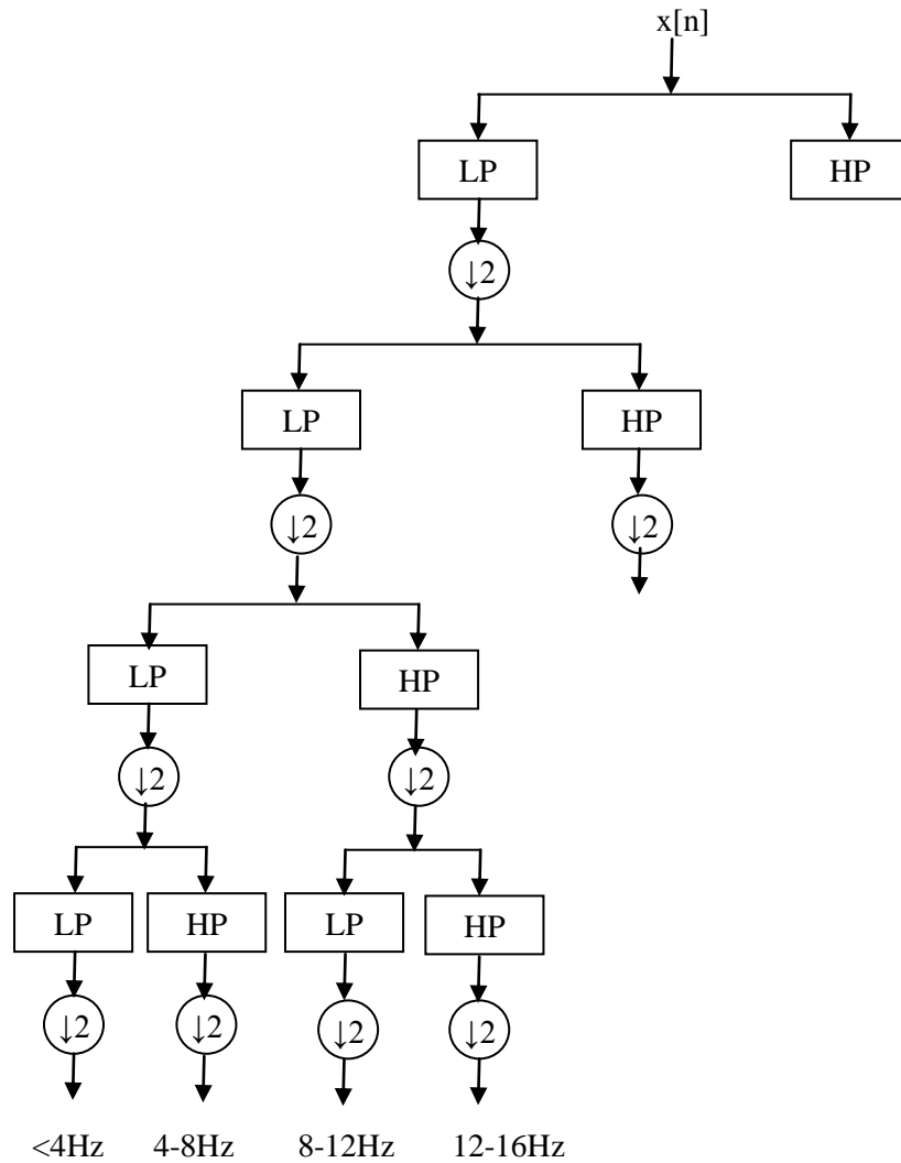
Figure 7.2: Wavelet decomposition to four levels, based on wavelet packet decomposition. Decomposition to basic EEG frequency bands is obtained.
