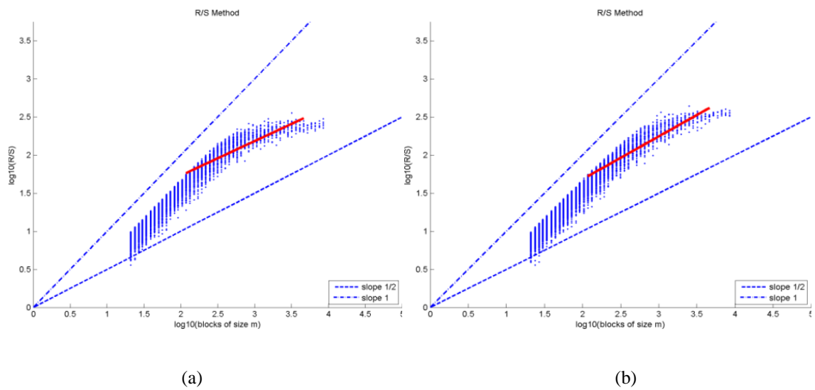
Figure 8.5: R/S estimation of the Hurst exponent, channel C4, for (a) quiet and (b) active sleep stage.
