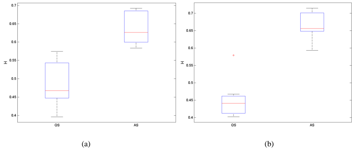
Figure 8.12: Values of the Hurst exponent, estimated for each EEG channel, for quiet and active sleep stages, for (a) subject 17 and (b) subject 20.
