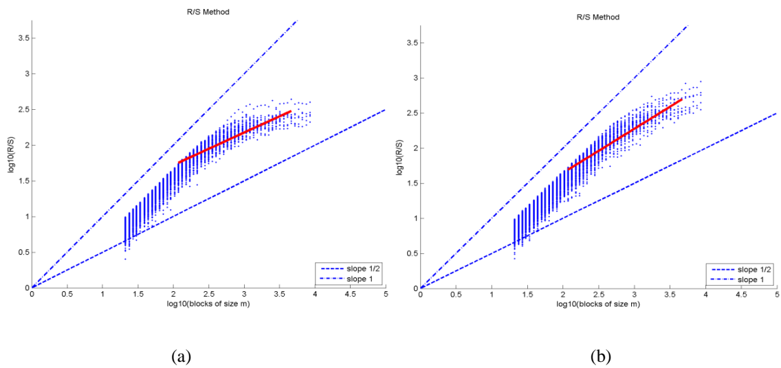
Figure 8.3: R/S estimation of the Hurst exponent, channel T3, for (a) quiet and (b) active sleep stage.
