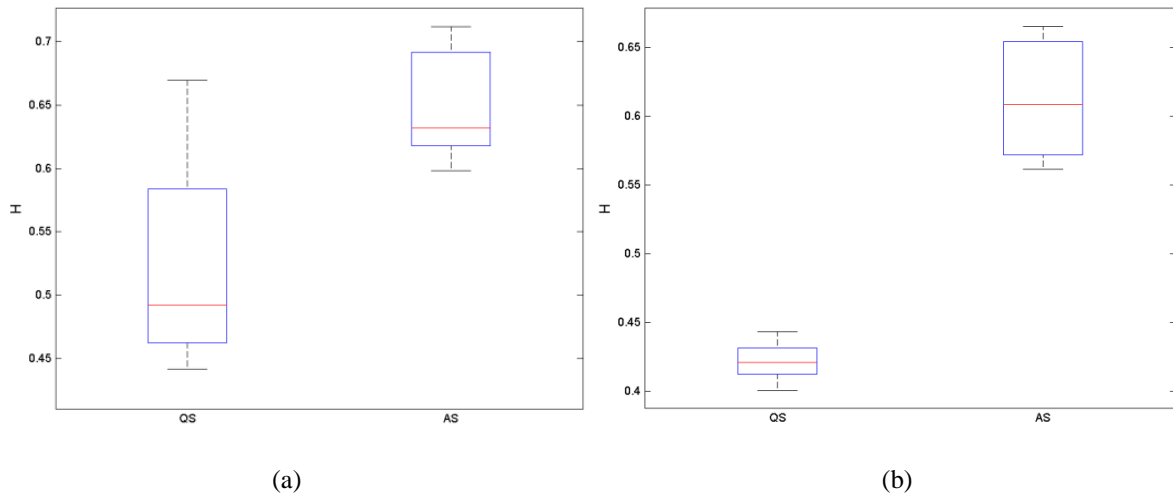
Figure 8.11: Values of the Hurst exponent, estimated for each EEG channel, for quiet and active sleep stages, for (a) subject 9 and (b) subject 15.
