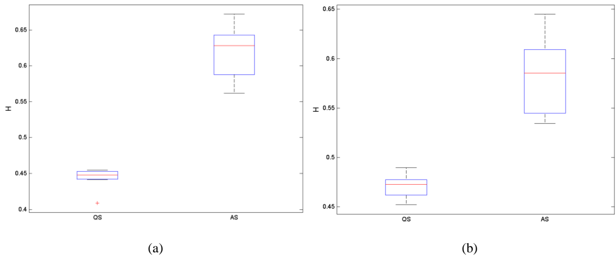
Figure 8.9: Values of the Hurst exponent, estimated for each EEG channel, for quiet and active sleep stages, for (a) subject 3 and (b) subject 4.
