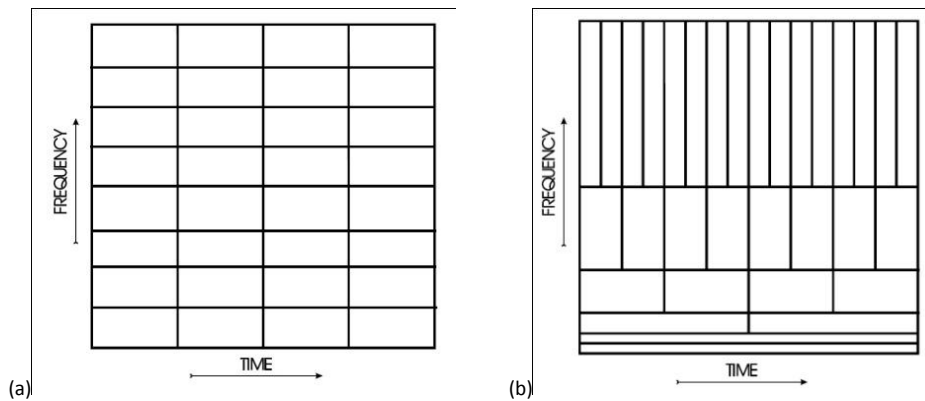
Figure 4.4: Symbolic division of time-frequency space for (a) STFT and (b) WT.
