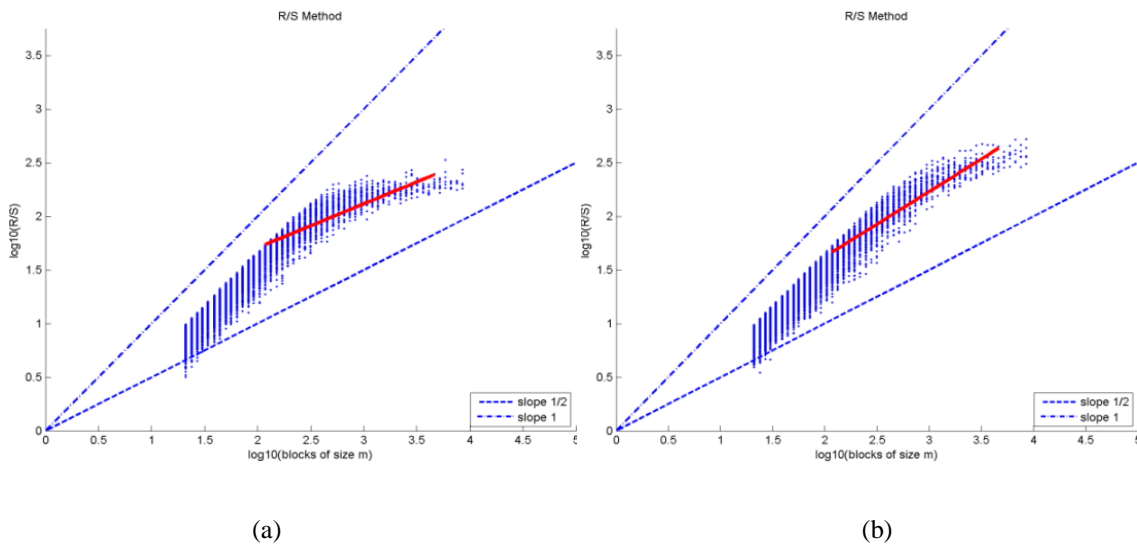
Figure 8.7: R/S estimation of the Hurst exponent, channel O1, for (a) quiet and (b) active sleep stage.
