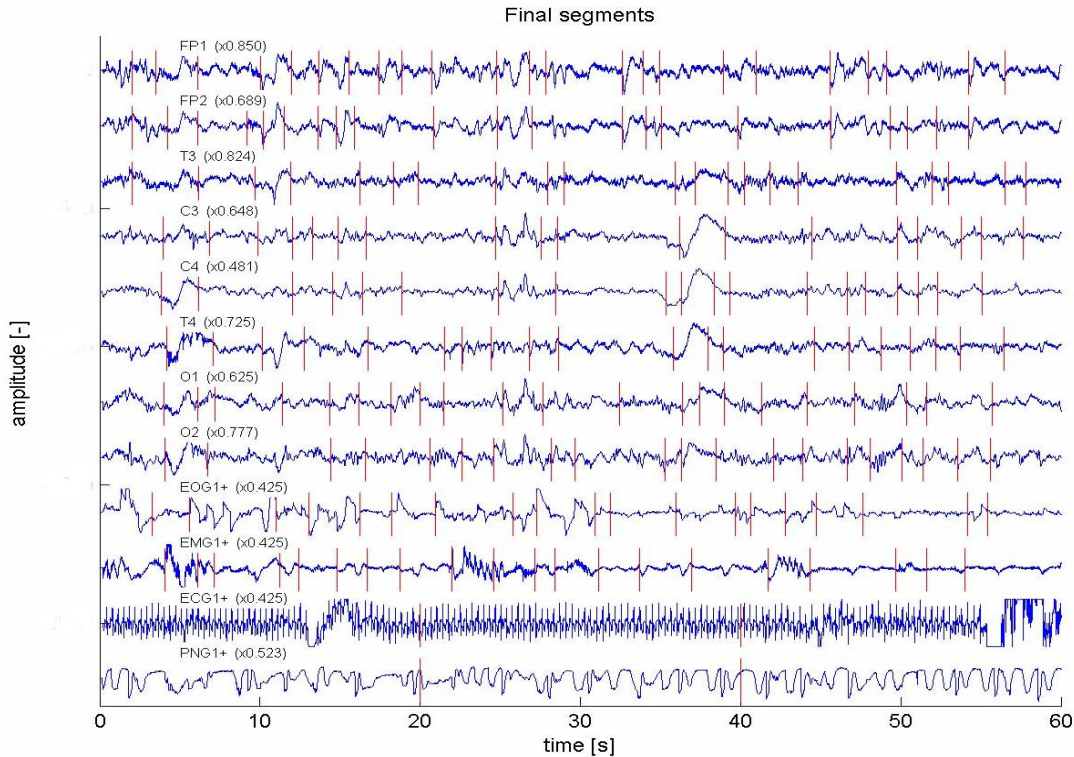
Figure 4.2: Final segmentation results of 60s of newborn PSG recording: adaptive segmentation was applied to EEG, EOG and EMG channels, while ECG and PNG channels were segmented to segments of constant length.
