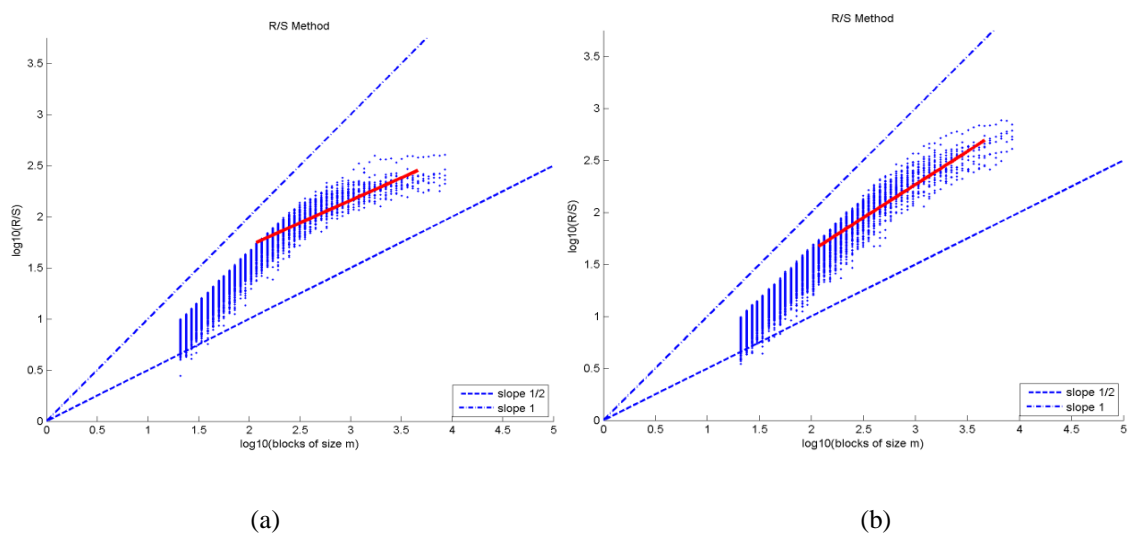
Figure 8.6: R/S estimation of the Hurst exponent, channel T4, for (a) quiet and (b) active sleep stage.
