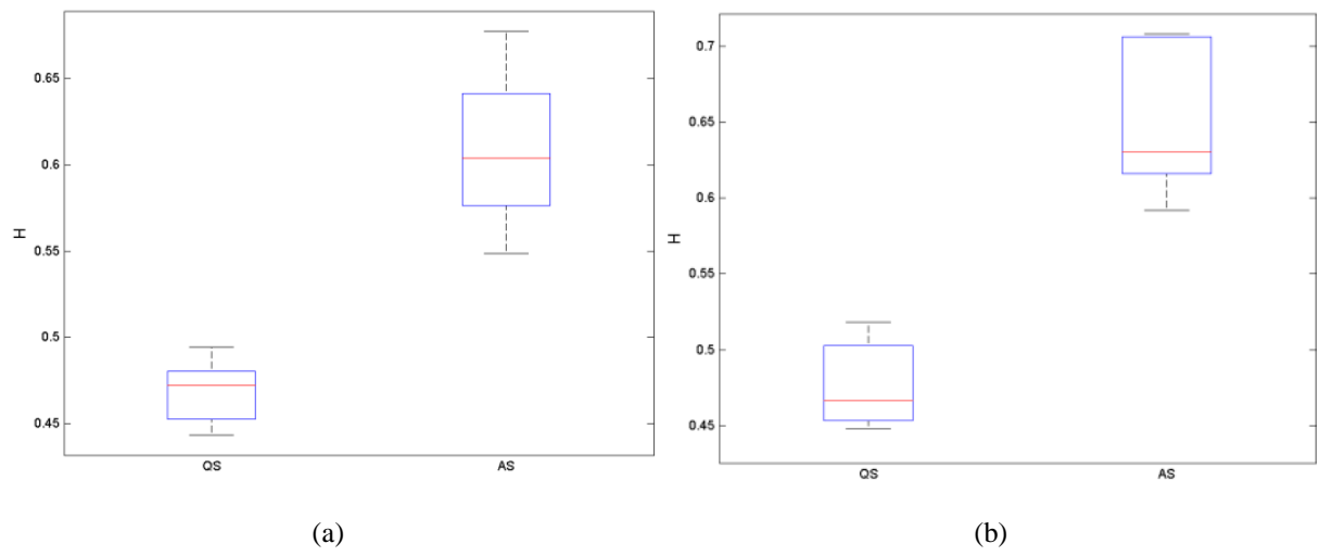
Figure 8.10: Values of the Hurst exponent, estimated for each EEG channel, for quiet and active sleep stages, for (a) subject 5 and (b) subject 8.
