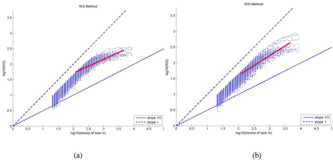
Figure 8.8: R/S estimation of the Hurst exponent, channel O2, for (a) quiet and (b) active sleep stage.
