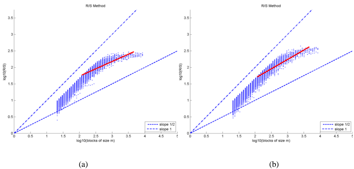
Figure 8.4: R/S estimation of the Hurst exponent, channel C3, for (a) quiet and (b) active sleep stage.
