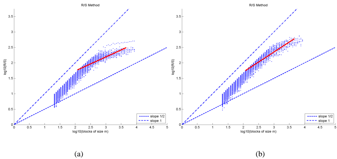
Figure 8.2: R/S estimation of the Hurst exponent, channel Fp2, for (a) quiet and (b) active sleep stage.
