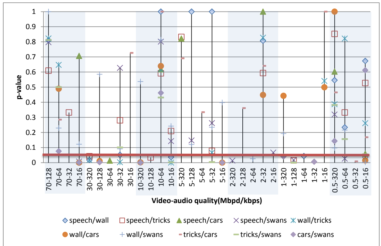
Fig 5.8 T-test results
