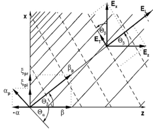
Fig. 2. Sketch of the leaky-wave field distribution approximated by the nonuniform wave (2) represented by solid lines of constant amplitude and by dashed lines of constant phase together with the decomposition of the wave and the field vectors. The angle \Theta_\beta represents \Theta_\beta^{(7)} defined in (7).
