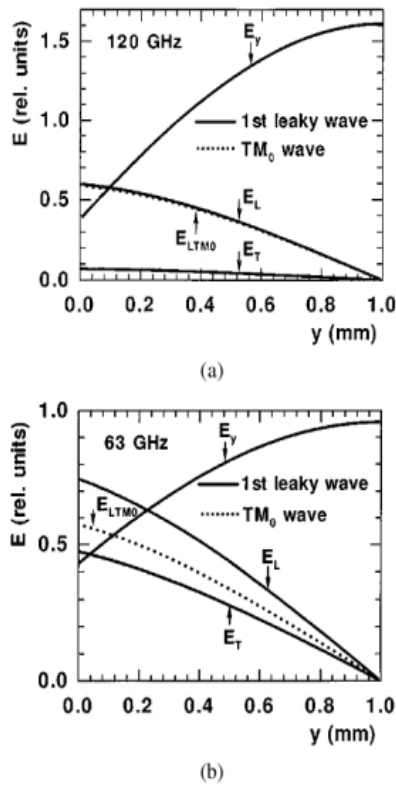
Fig. 4. Field distribution of the first leaky wave and the TM_0 surface wave across the substrate at the point x = 7.5 mm, z = 0 mm and at a frequency of: (a) 120 GHz and (b) 63 GHz. E_{LTM_0} denotes the E_L -field component of the TM_0 surface wave.
