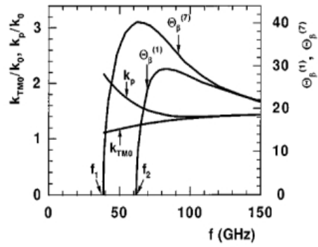
Fig. 3. Phase constant and angle of propagation of the partial waves approximating the first leaky wave on the slotline from Fig. 1.
