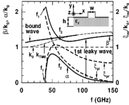
Fig. 1. Dispersion characteristics and the Green function pole position of the lossless slotline when w = h = 1 mm and \epsilon_r = 2.25 .
