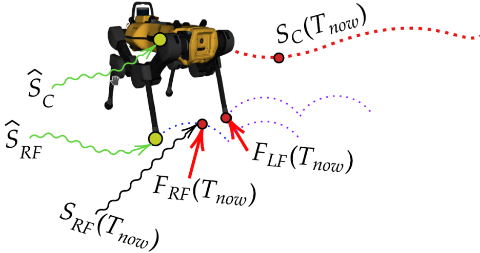
Figure 2.5: The WBC tracking controller is tasked to track the optimized state trajectory S_{(\cdot)}(t) , taking the current state \hat{S}_{(\cdot)} and optimized ground reaction forces into account.
