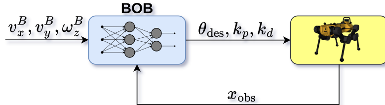
Figure 2.6: Overview of BobController’s architecture
