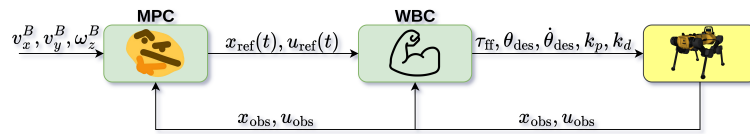
Figure 2.3: Overview of MpcController 's architecture
