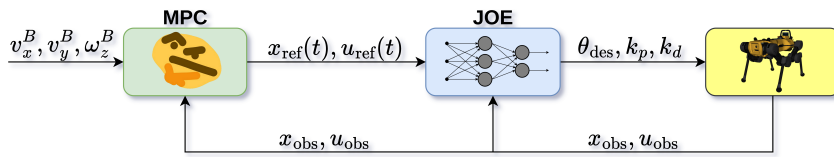
Figure 2.8: Overview of JoeController's architecture
