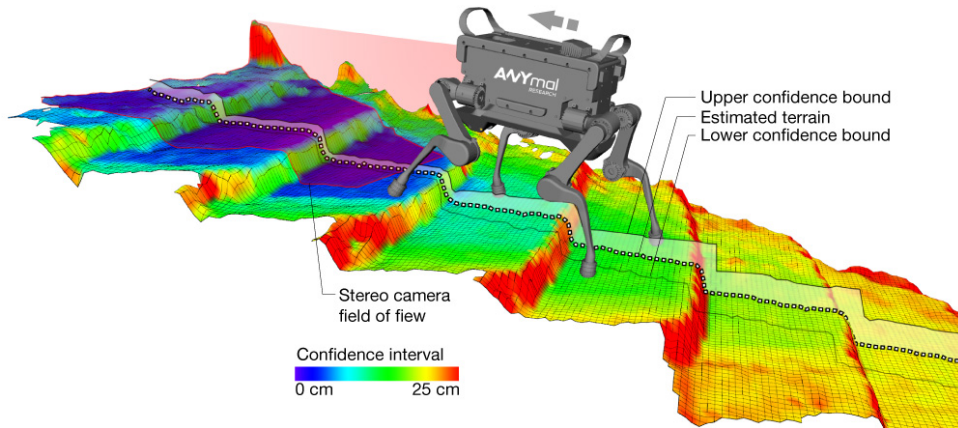
Figure 1.2: Gridmap [5]
