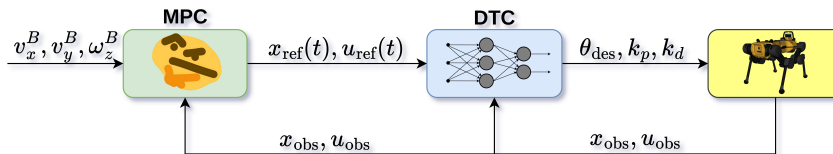
Figure 2.7: Overview of DtcController’s architecture
