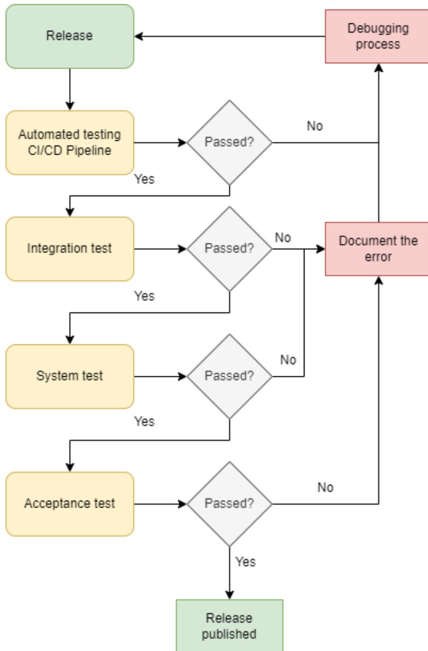
Figure 2.8: Internal release - Test workflow
