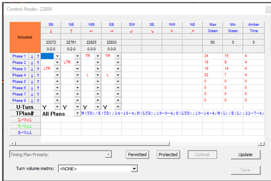
Figure 14: Signal Plan Set-up Interface, source: DynuStudio Software
