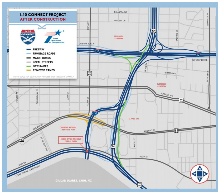
Figure 2: I-10 Connect After Reconstruction, source: TxDOT, I-10 Connect
