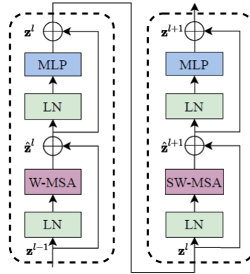
■ Figure 4.3 Two consecutive Swin Transformer blocks - W-MSA and SW-MSA are regular and shifted window multi-head self attention modules, MLP is multi-layer perceptron also called feed-forward network.[41]
