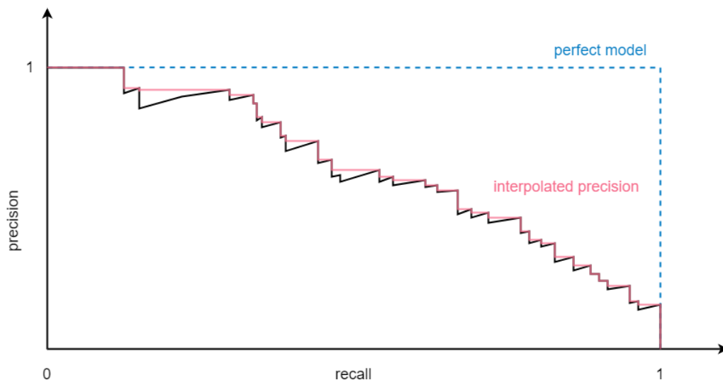
■ Figure 6.2 Precision-Recall curve (black), interpolated PR curve (pink), PR curve for a perfect model (blue).
