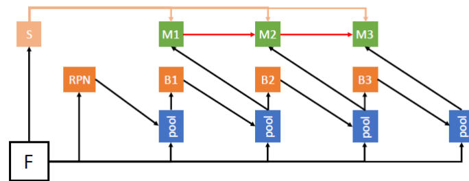
■ Figure 6.7 Hybrid Task Cascade (HTC) framework: “F” stands for input, “RPN” for region proposal network network, “pool” region-wise feature extraction, “B” bounding box regressor, “M” mask branch, and “S” semantic segmentation branch.[51]
