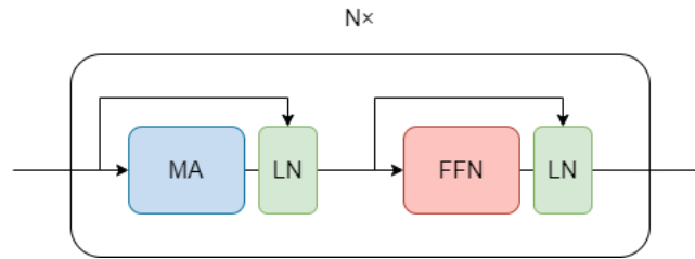
■ Figure 4.1 A diagram of one layer within the encoder of a transformer - MA: multi-head attention, LN: layer normalization, FFN: feed-forward network.[37]
