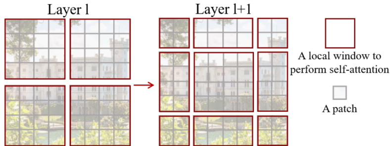
■ Figure 4.4 Shifted windows algorithm. Layer l + 1 uses shifted windows partitioning that provides connections between the boundaries of previous windows.[41]
