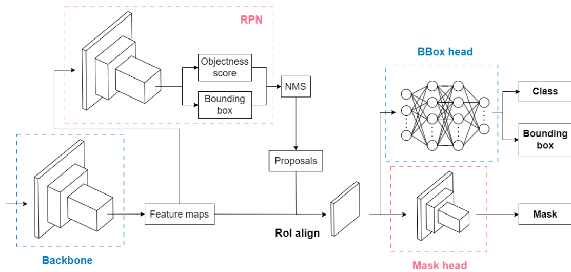
■ Figure 6.1 Instance segmentation architecture overview (Mask R-CNN[47]).
