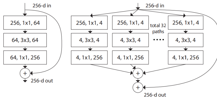
■ Figure 3.3 Left: a ResNet block, Right: a ResNeXt block with cardinality = 32.[36]
