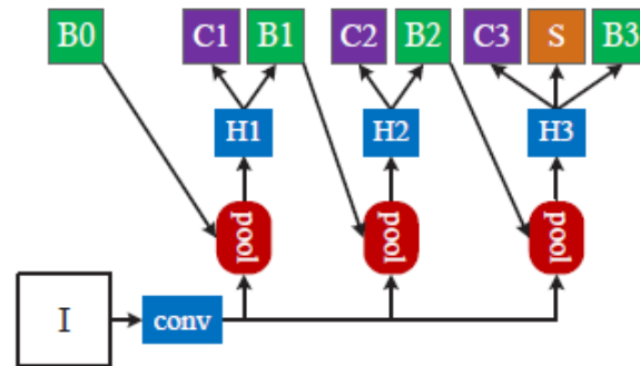
■ Figure 6.5 Architecture of Cascade R-CNN framework “I” is input image, “conv” backbone convolutions, pool” region-wise feature extraction, “H” network head, “B” bounding box, “S” segmentation branch and “C” classification. “B0” is proposals. [50]
