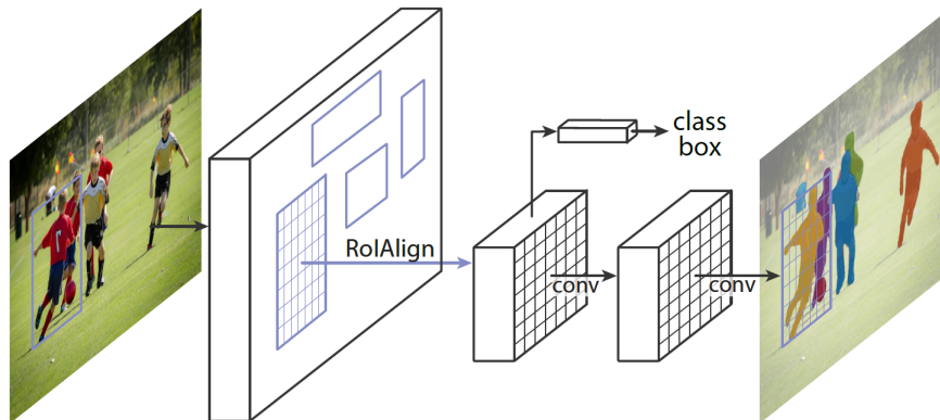
■ Figure 6.3 Mask R-CNN framework - Faster R-CNN with addition of the RoIAlign operation and a branch for semantic segmentation on RoIs.[47]
