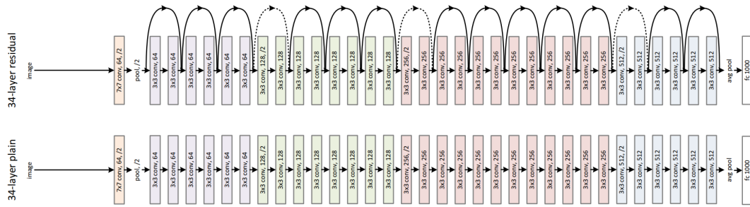
■ Figure 3.2 Bottom: a plain network with 34 layers, Top: ResNet with 34 layers.[35]
