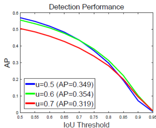
■ Figure 6.4 Decreasing AP for detectors trained with different IoU threshold u . [50]
