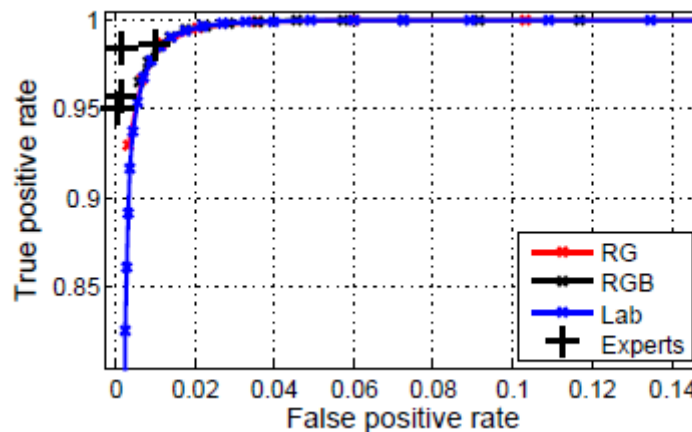
■ Figure 2.1 ROC calculated for linear classifier using all testing images and different color spaces. It compares the performance of the model with the performance of experts.[4]
