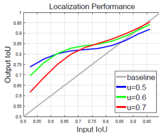
■ Figure 6.6 Output IoU of a regressor is almost always higher than the input IoU. [50]
