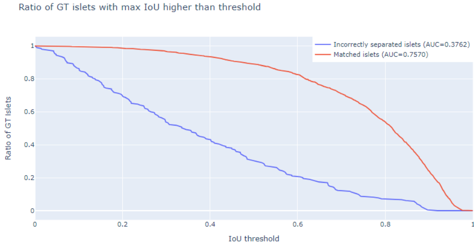
Figure 8.2 The GT ratio over IoU metric for the IsletNet model demonstrates a significantly higher area under the curve (AUC) for islets classified as matched, contrasting with incorrectly separated islets that exhibit notably lower IoU values.
