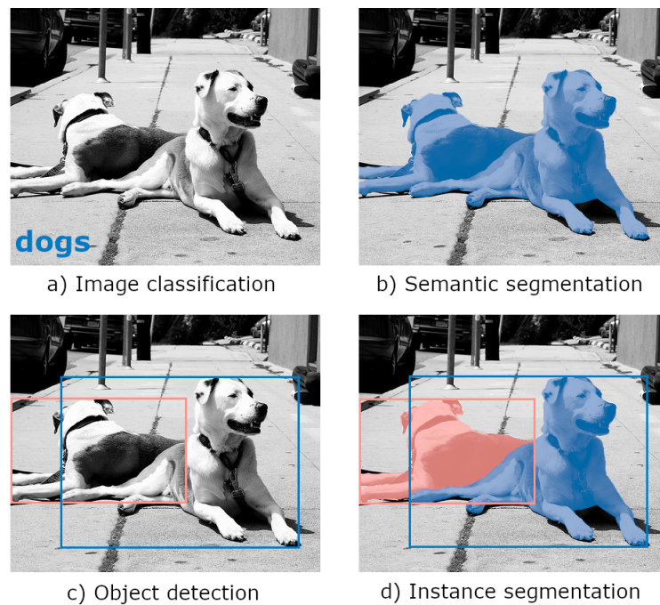
■ Figure 3.1 Computer vision tasks: a) image classification, b) semantic segmentation, c) object detection, d) instance segmentation. Image is from the COCO 2017 dataset[34], modified.
