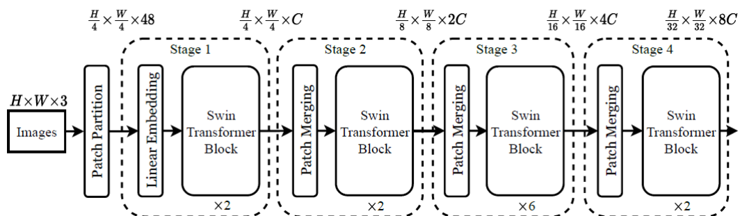
■ Figure 4.2 Swin Transformer architecture[41]
