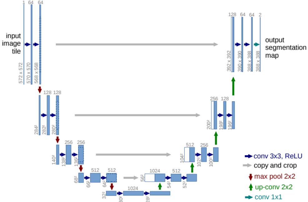
■ Figure 5.1 UNet architecture.[30]
