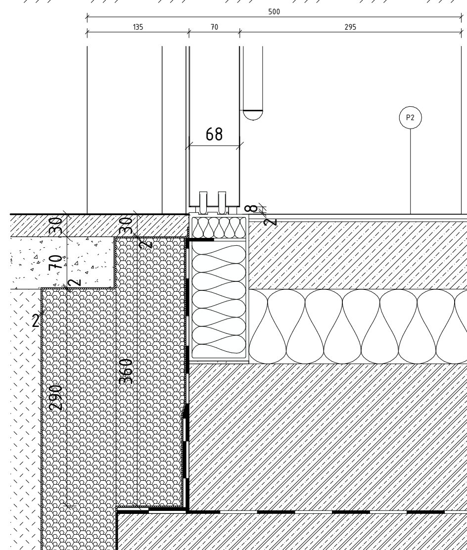
DETAIL 8, M 1:5
