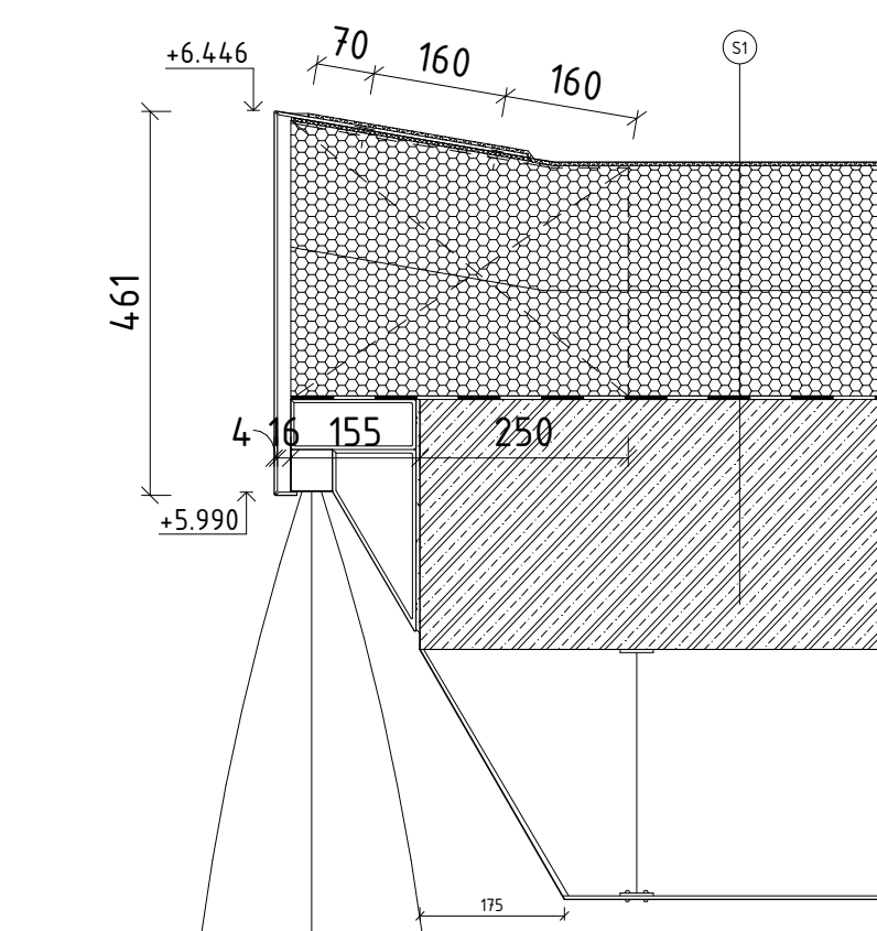
DETAIL 7, M 1:10
