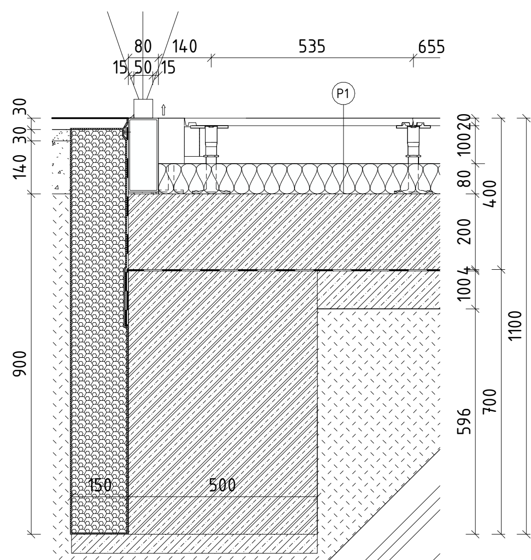
DET6 - detail soklu LOP
