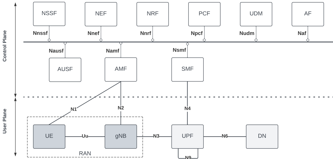
Figure 2.2. 5G system architecture [13].
