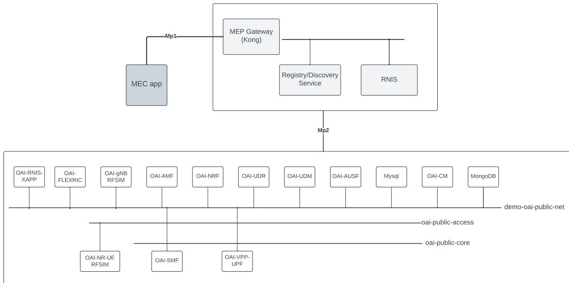
Figure 3.7. Technical overview of OAI-MEP [26].
