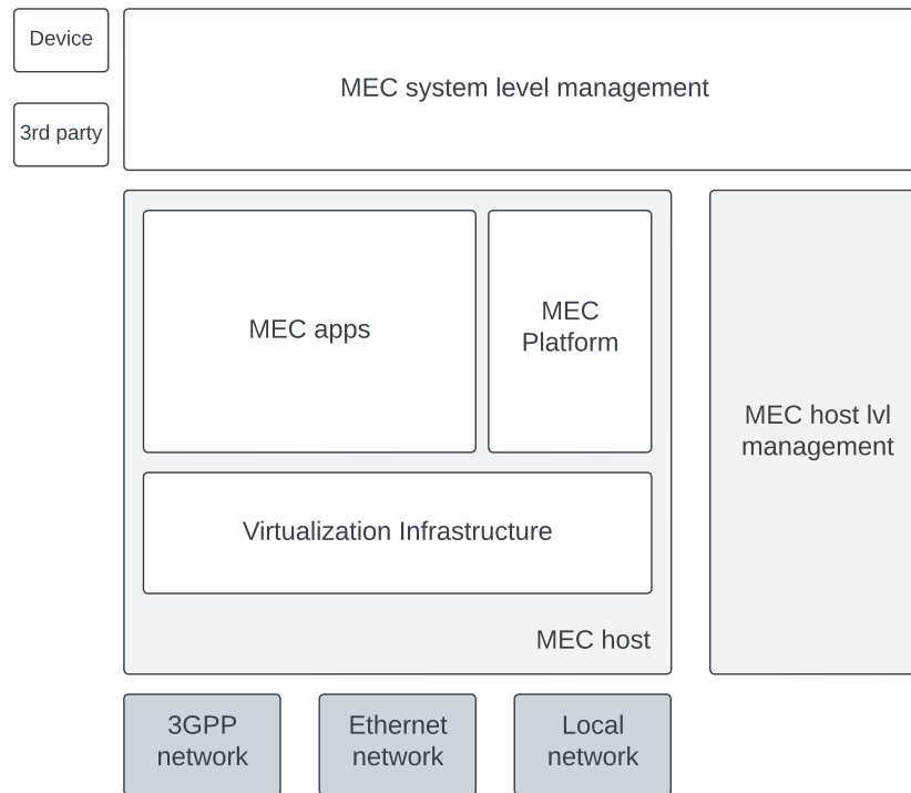
Figure 2.6. ETSI MEC framework [15].
