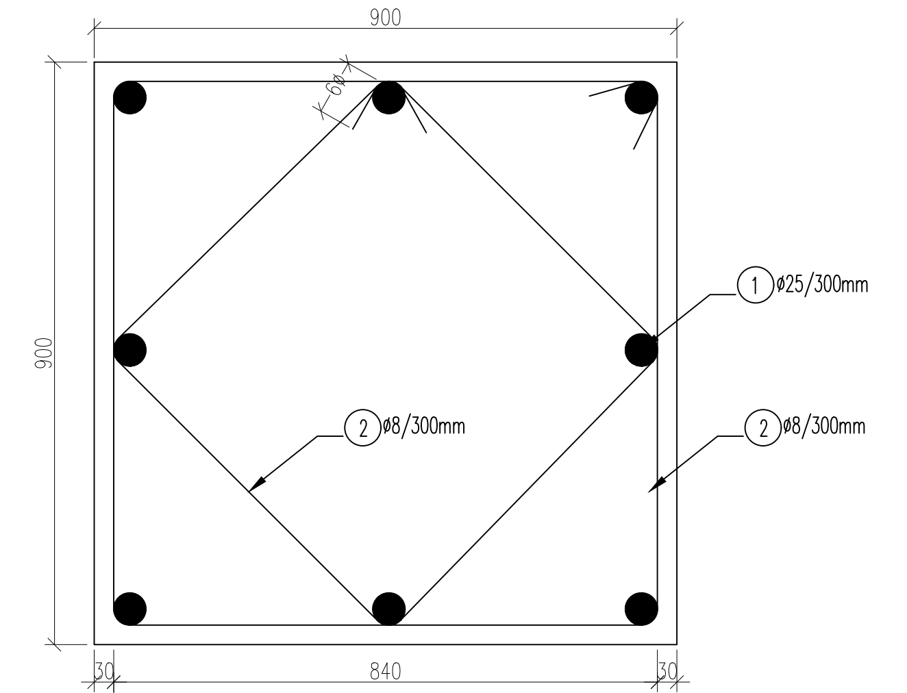
SECTION 1-1 (M 1:10)
