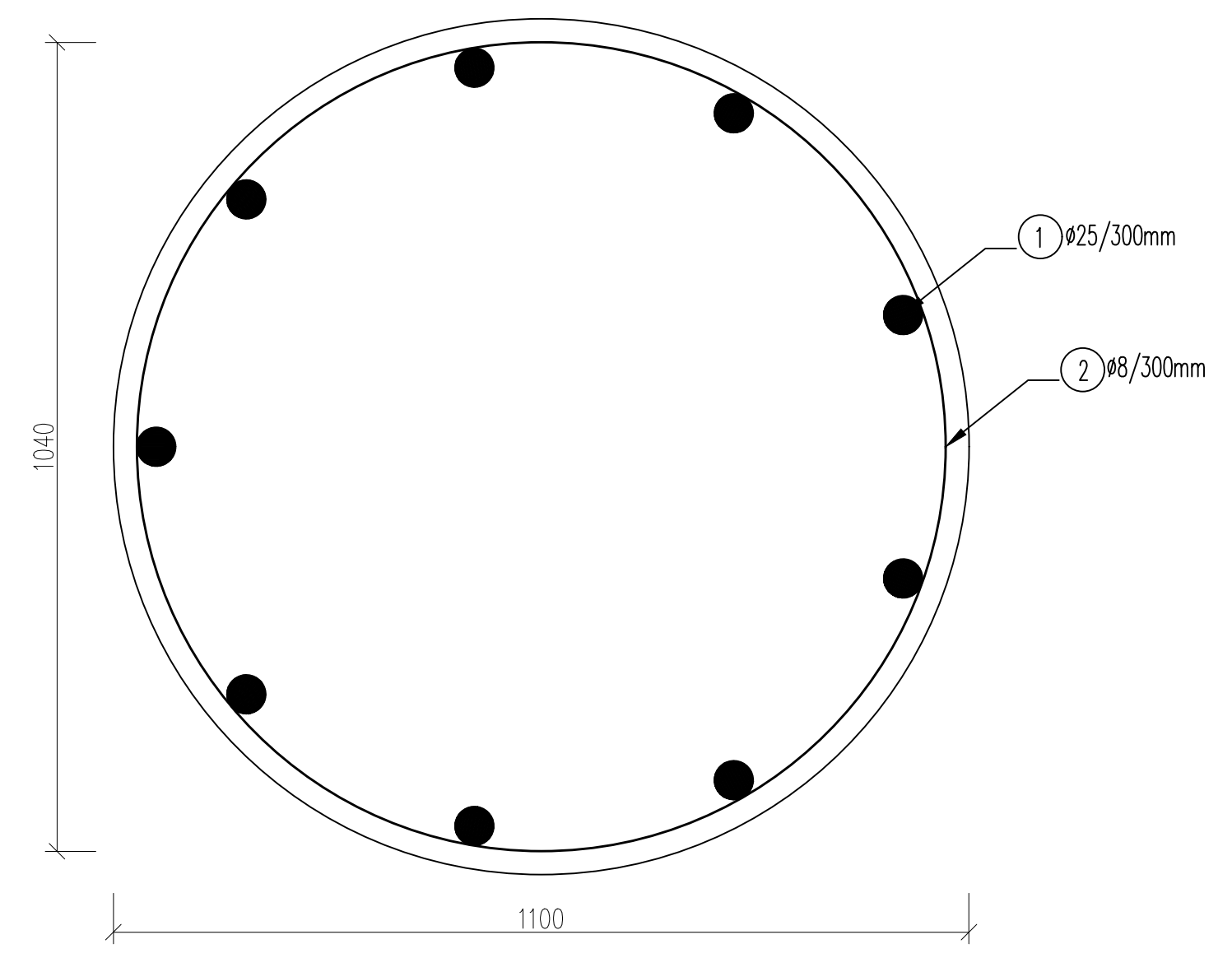
SECTION 1-1 (M 1:10)
