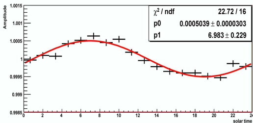
Figure 6: One-dimensional projection in right ascension of the two-dimensional CR sky map in local solar time. The red line shows the best-fit to ARGO-YBJ data (crosses).
