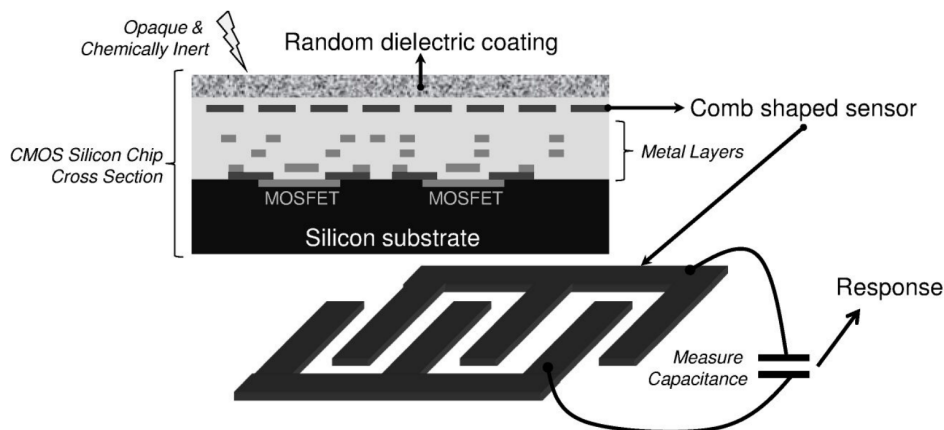
■ Figure 1.10 Construction of a coating PUF [5]
