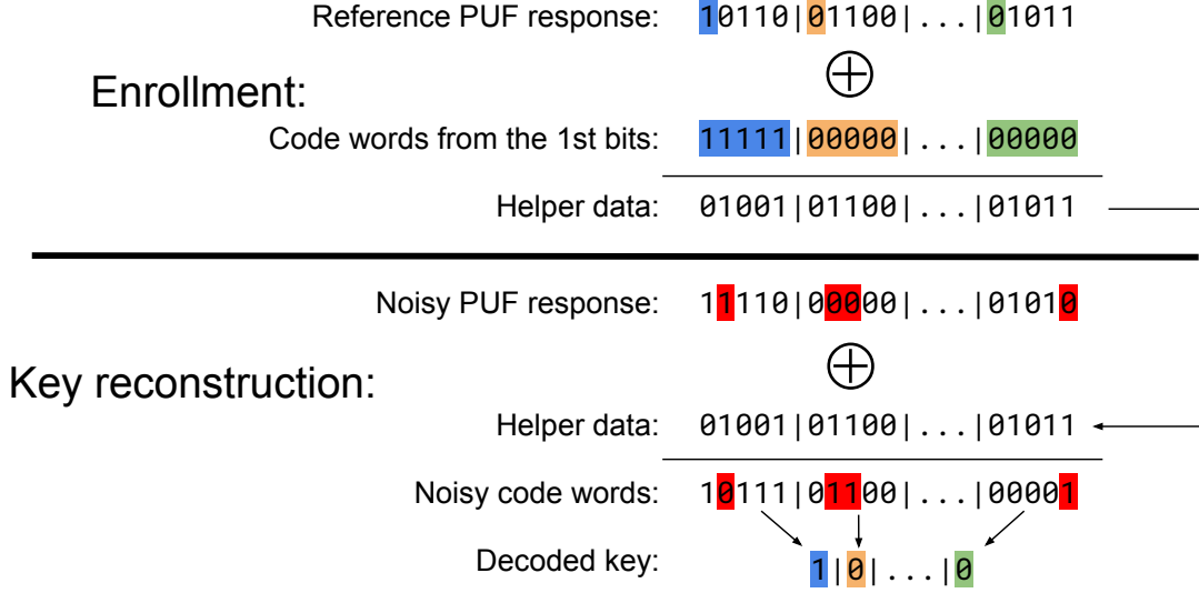
■ Figure 5.1 An example of enrollment and key reconstruction phases for a repetition code of length 5. Red bits are the error bits (flipped compared to the reference response), other colors represent individual bits of the key. [6]
