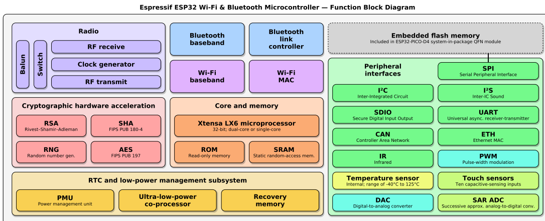
■ Figure 3.2 ESP32 chip function block diagram [47]
