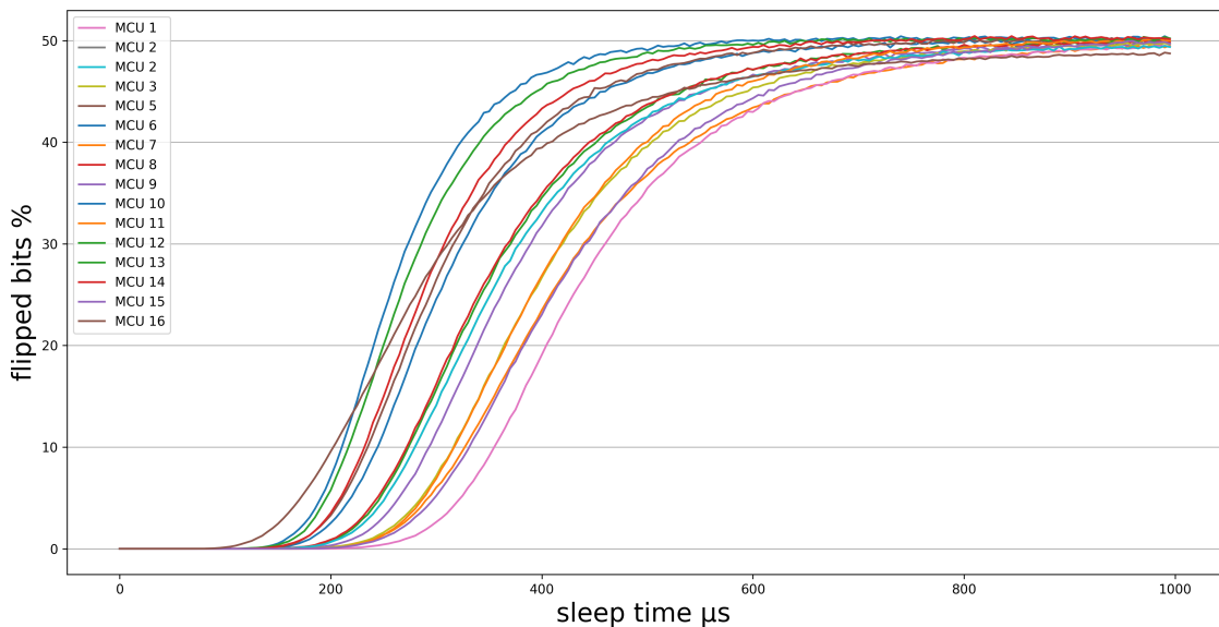
■ Figure 4.2 Percentage of flipped bits of all MCUs at 20 °C (RTC SRAM method)
