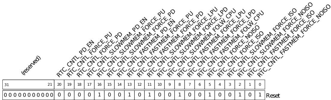
■ Figure 4.1 RTC domain power management register (address 0x3FF48080) [45]
