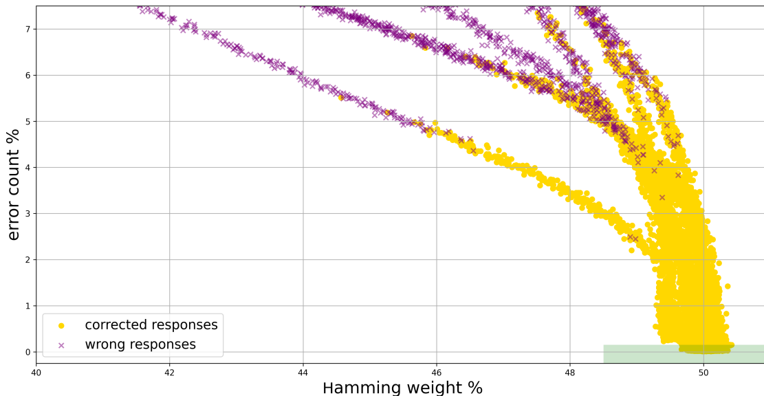
■ Figure 5.3 A scatter plot showing the effect of Hamming weight and error count on correct response reconstruction. The green region represents data points where the RTC SRAM response is accepted as a valid response. Data obtained from MCUs 1–6. RTC SRAM method with 10 mS turn off interval was used.
