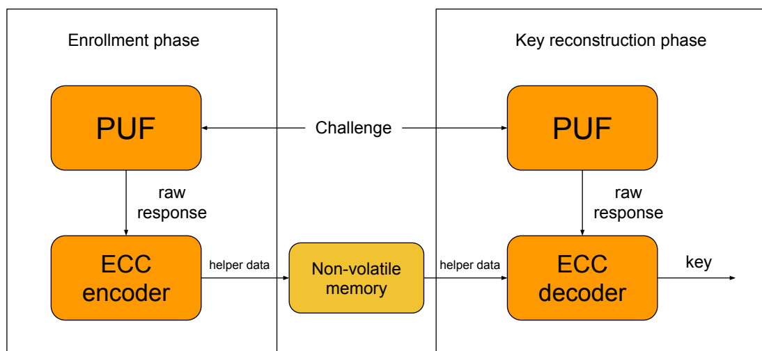
■ Figure 1.7 PUF-based key generation mechanism, inspired by [25]
