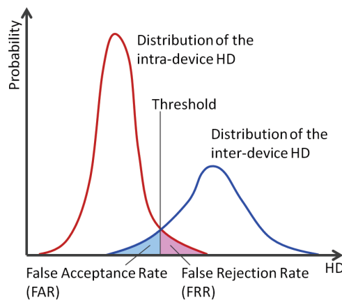
■ Figure 1.5 PUF identification: intra and inter HD distributions [20]
