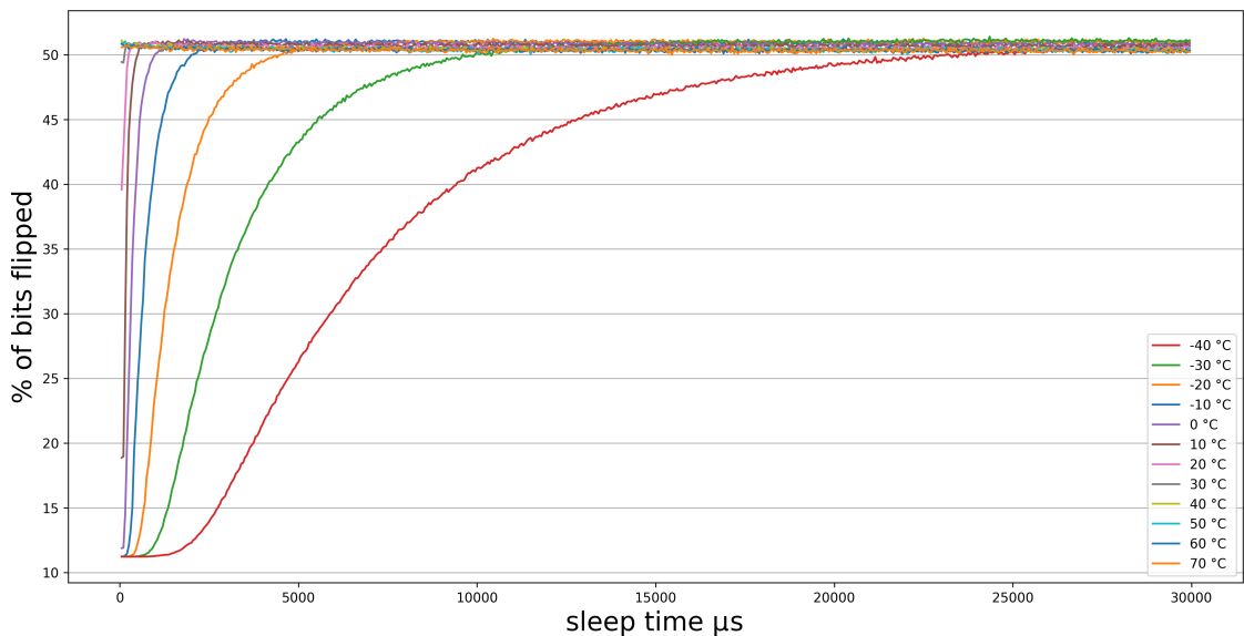
■ Figure 4.6 Percentage of flipped bits of MCU 6 across a range of temperatures (deep sleep method)
