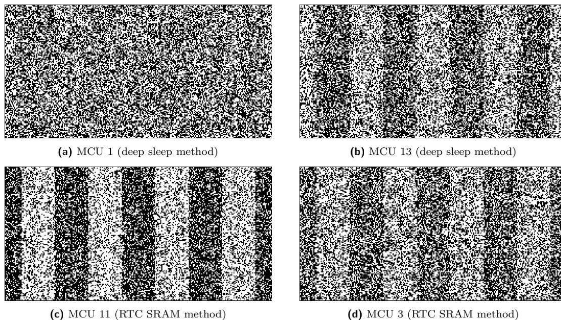
■ Figure 4.7 Visualization of PUF responses from different MCUs in a 256 \times 128 bit grid
