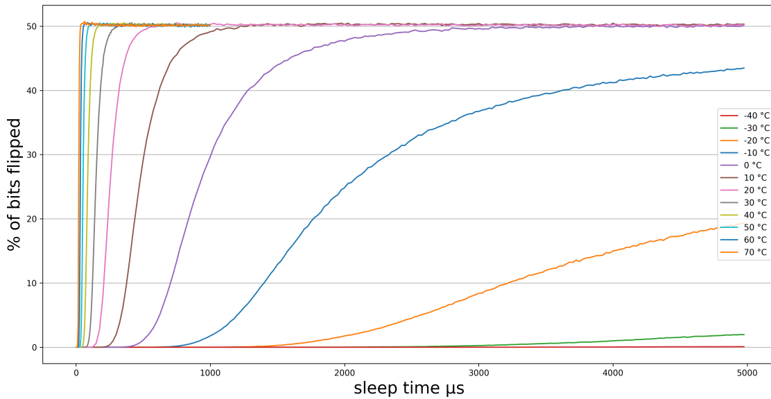
■ Figure 4.3 Percentage of flipped bits of MCU 6 across a range of temperatures (RTC SRAM method)
