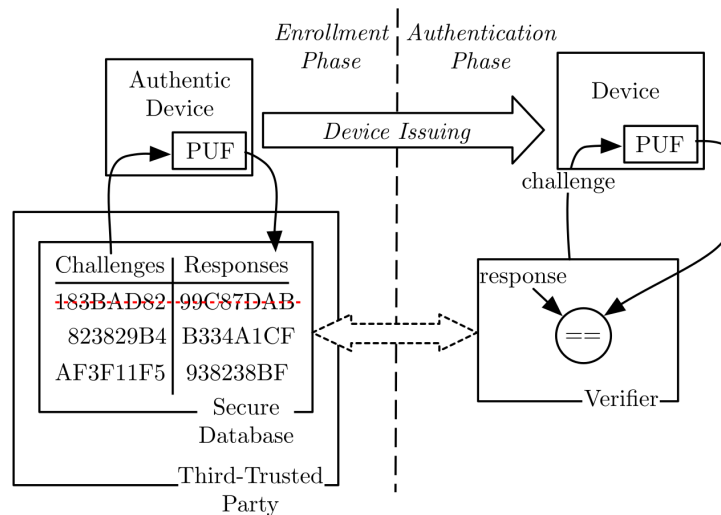
■ Figure 1.6 PUF-based authentication protocol [22]
