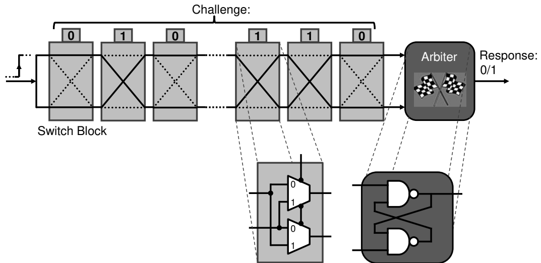
■ Figure 1.9 Construction of an arbiter PUF as proposed by [30], image from [5]
