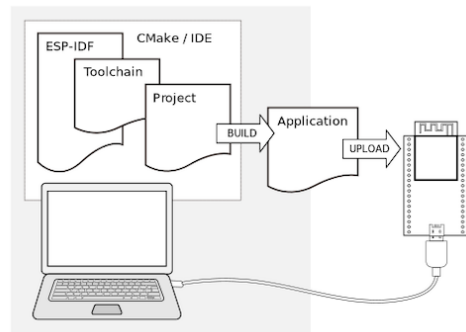
■ Figure 3.3 Development of applications for ESP32. [44]
