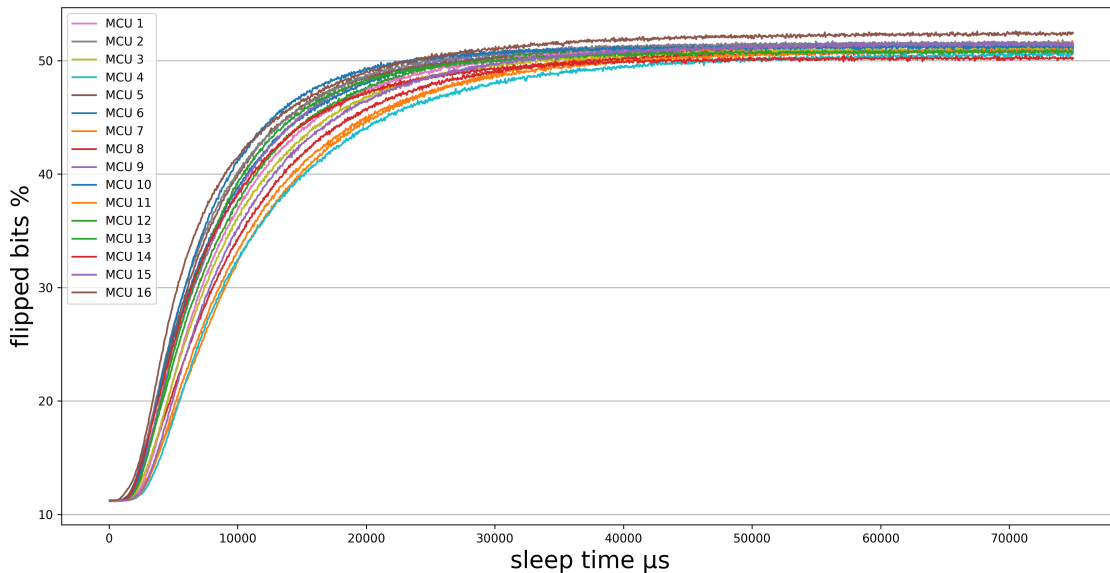
■ Figure 4.5 Percentage of flipped bits of all MCUs at -40 °C (deep sleep method)
