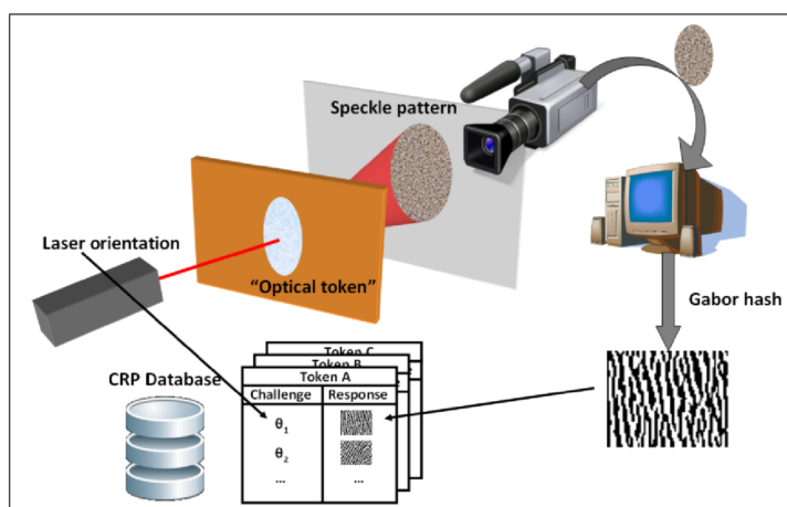
■ Figure 1.8 Operation of the optical PUF
