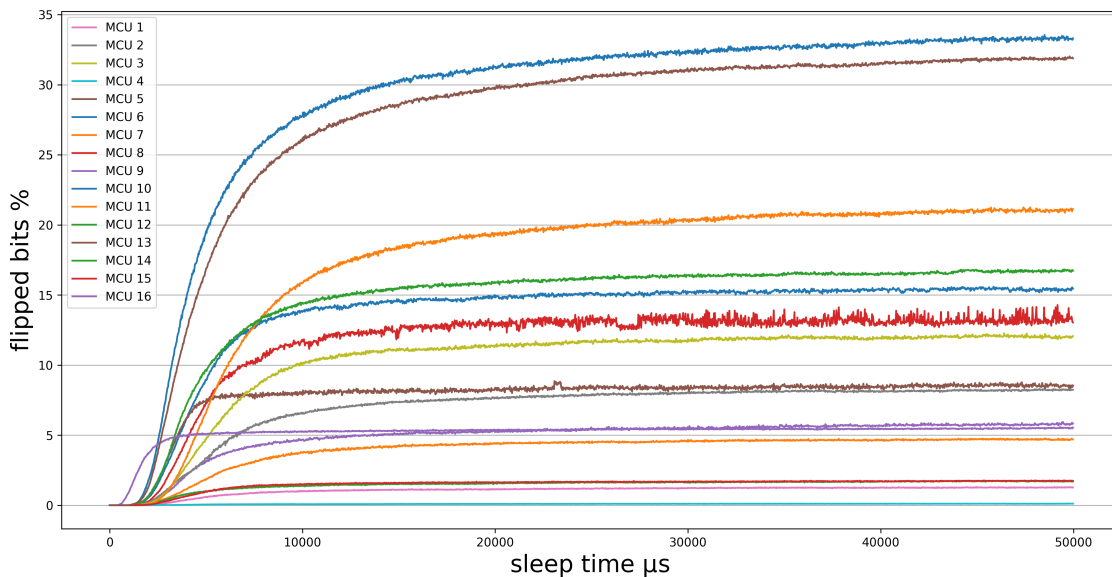
■ Figure 4.4 Percentage of flipped bits of all MCUs at -20 °C (RTC SRAM method)
