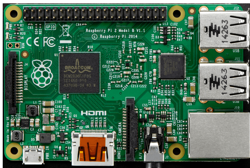
Figure 4.4. The physical appearance of the specific RaspberryPi used in the PMSM control demonstration for Simulink/pysimCoder. Produced in 2014, it is a Model 2B (v1.1).
