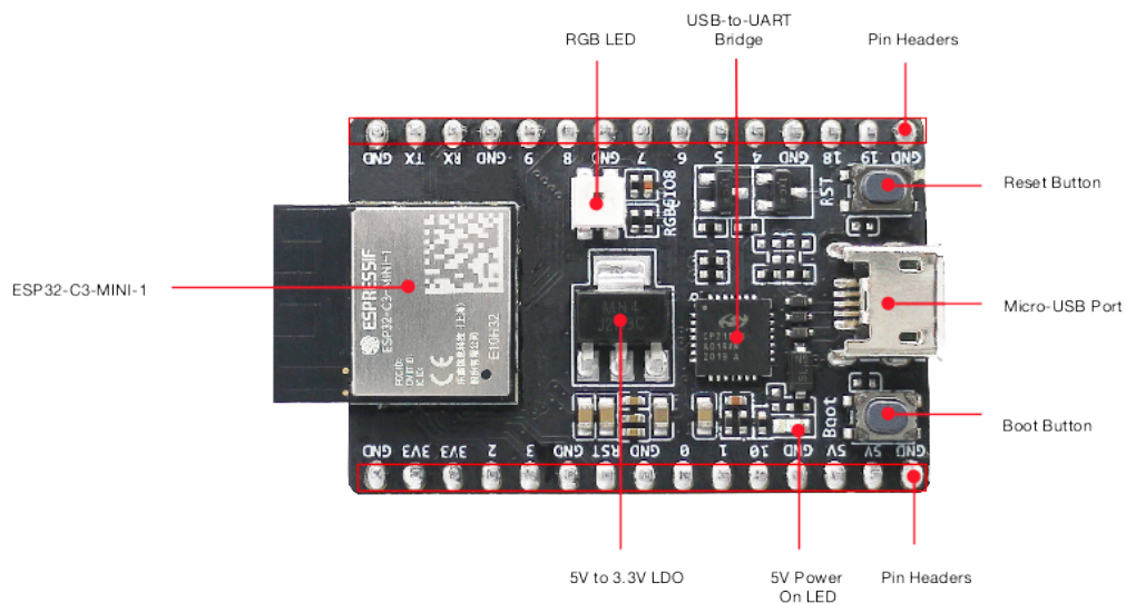
Figure 5.1. The different components of the ESP32C3-DevKitM-1 board are presented with labels. On the left is the main chip, while on the right is the micro-USB connection. The pin headers can be found on the top and bottom. Other components include RGB LED, Reset and Boot buttons, 5V to 3.3V LDO and more.
