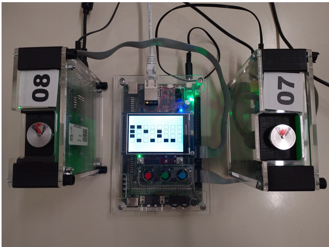
Figure 4.2. The two motors are connected to the Zynq board, while the knobs are used to tune the PID controller. Both the motors are in the same position, which is the desired output of this diagram.
