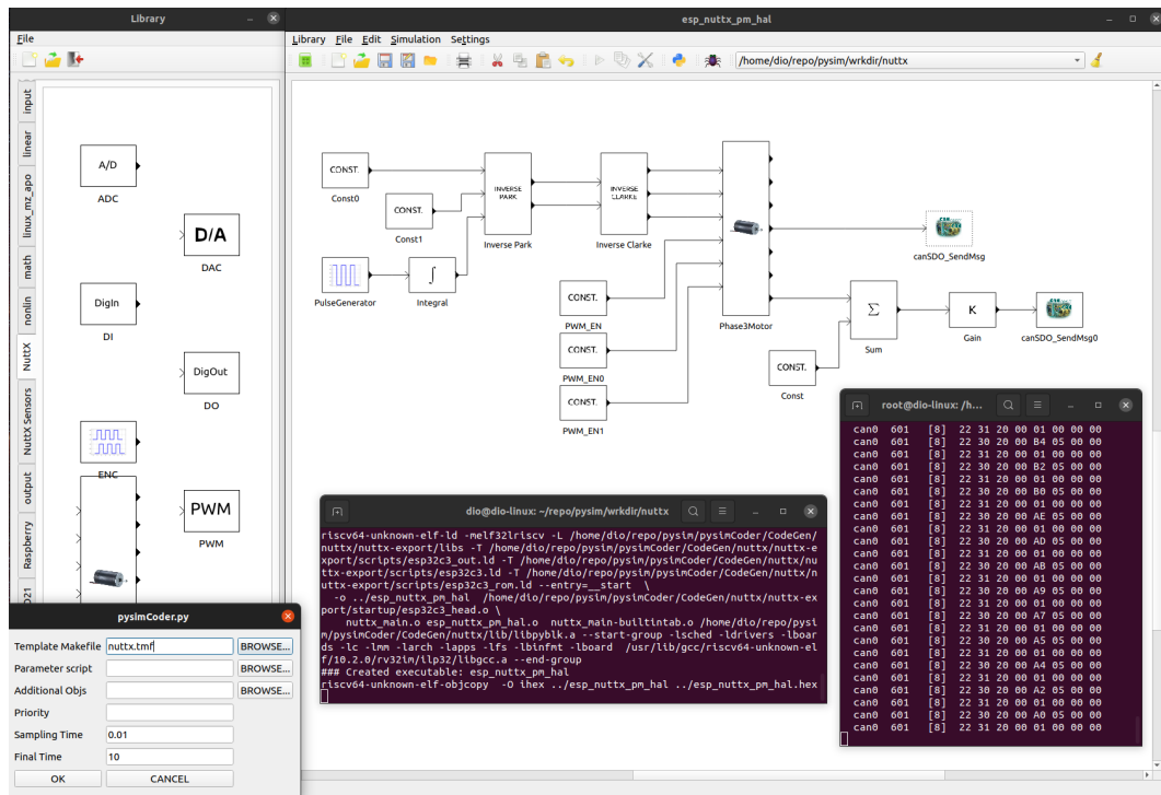
Figure 5.4. Screenshot demonstrating motion control of 3-Phase PMSM using ESP32C3 with NuttX RTOS. Terminal on right shows a CAN receiver printing in hexadecimal format, which represents the actual location from IRC input, and sector value obtained from the HAL sensors on the motor. The window in the middle is for pysimCoder terminal output. Diagram is similar to RaspberryPi PMSM motion control demo, but uses CAN instead of TCP for communication.
