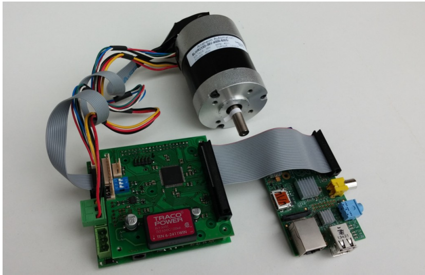
Figure 4.5. Hardware setup for motion control of 3-phase motor (PMSM) using RaspberryPi board and Simulink. The motor is connected to the motor driver, the FPGA board is fitted on top of the driver, and the RaspberryPi is connected to the expansion board with a HAT cable module. Note that the board in this picture is one model older than the one used in my implementation.
