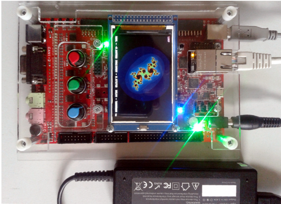
Figure 4.1. The hardware design of the MZ_APO kit is presented. Some main peripherals that can be noticed easily are the LCD screen, three rotary knobs, GPIO pins, LEDs, and the interfaces on the edges of the board. It is commonly used as educational kit for some courses in the Czech Technical University and was designed by Ing. Petr Porazil [14].
