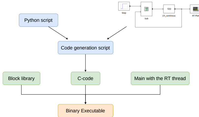
Figure 2.2. Code path from GUI to executable file, inspired by presentation from Prof. Roberto Bucher [10].
