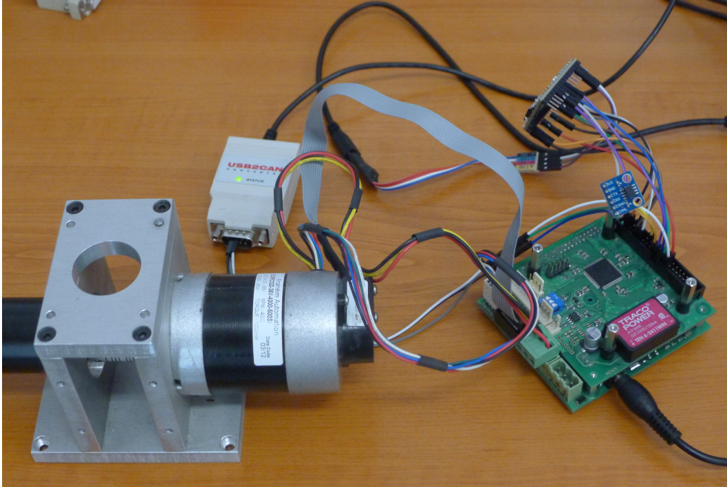
Figure 5.2. Hardware setup for 3-phase PMSM motion control using ESP32C3 with NuttX RTOS. Code for controlling the motor was generated by pysimCoder. Hardware connections are based from same demonstration for RaspberryPi.
