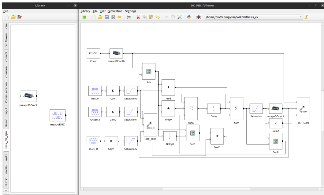
Figure 4.3. Three knob blocks control the PID values. One DC motor is fed by some constant value, while the other is connected in a negative feedback loop and controlled by a PID controller. The signals are sent through TCP for recording and graphing.
