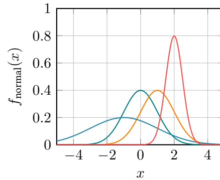
(b) The corresponding normal distributions of Y = \text{logit}(X) .
