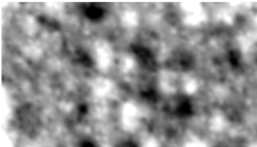
(c) Simplex noise fBm from eq. 3.4, with non-zero coordinate offset \vec{\sigma} \neq \vec{0} and parameters g = \frac{1}{l} = 1.5, k = 5 .
