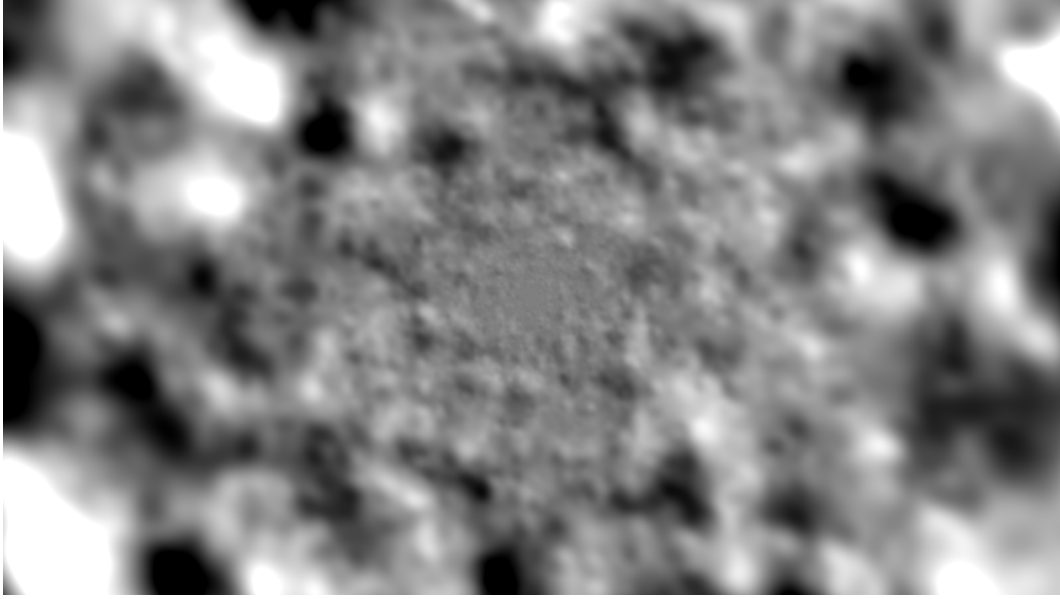
Figure 3.6: The final implementation of the blended fBm Simplex noise based on the distance to the center r , from eq. 3.12, with non-zero coordinate offset \vec{\sigma} \neq \vec{0} and parameters a = g = \frac{1}{7} = 1.5, k = 5 . Amplitude adjusted for visualization.
