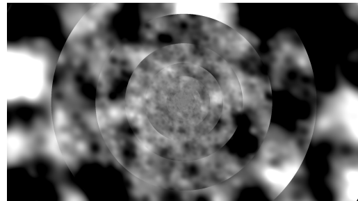
(d) Simplex noise fBm with index offsets based on the distance to the center r , from eq. 3.7, with non-zero coordinate offset \vec{\sigma} \neq \vec{0} and parameters a = g = \frac{1}{l} = 1.5, k = 5 .
