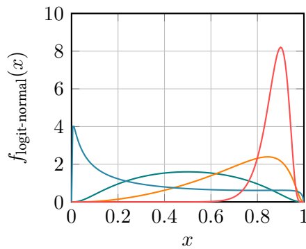
(a) Examples of logit-normal distributions of random variable X .
